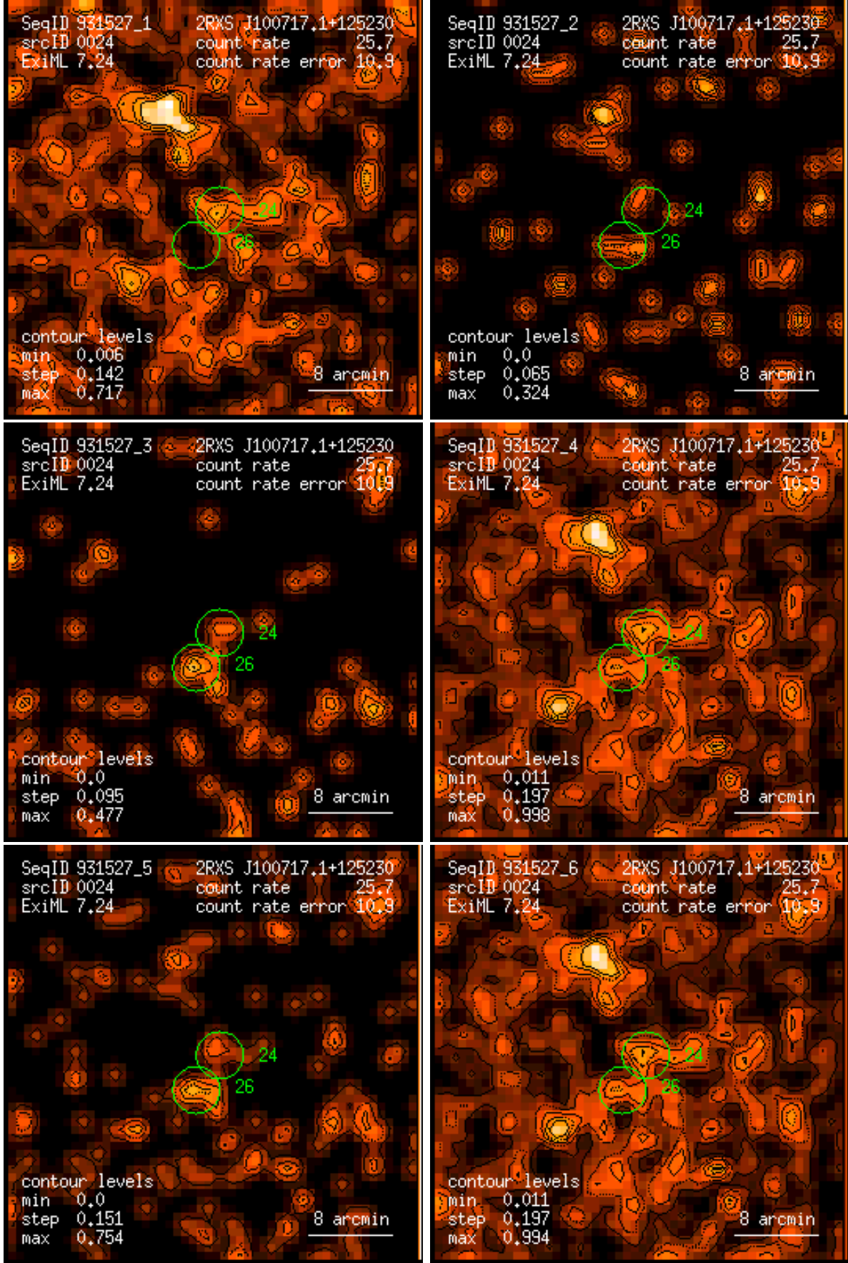
Figure 24: RASS 931527: detection 0024: band rate images, Gaussian filter: (1) PSPC channels 11 – 41, (2) 52 – 90, (3) 91 – 201, (4) 11 – 235, (5) 52 – 201, (6) 11 – 201. Broad band rates in counts/ks. Band rate contour levels in counts/ks/arcmin 2 .
