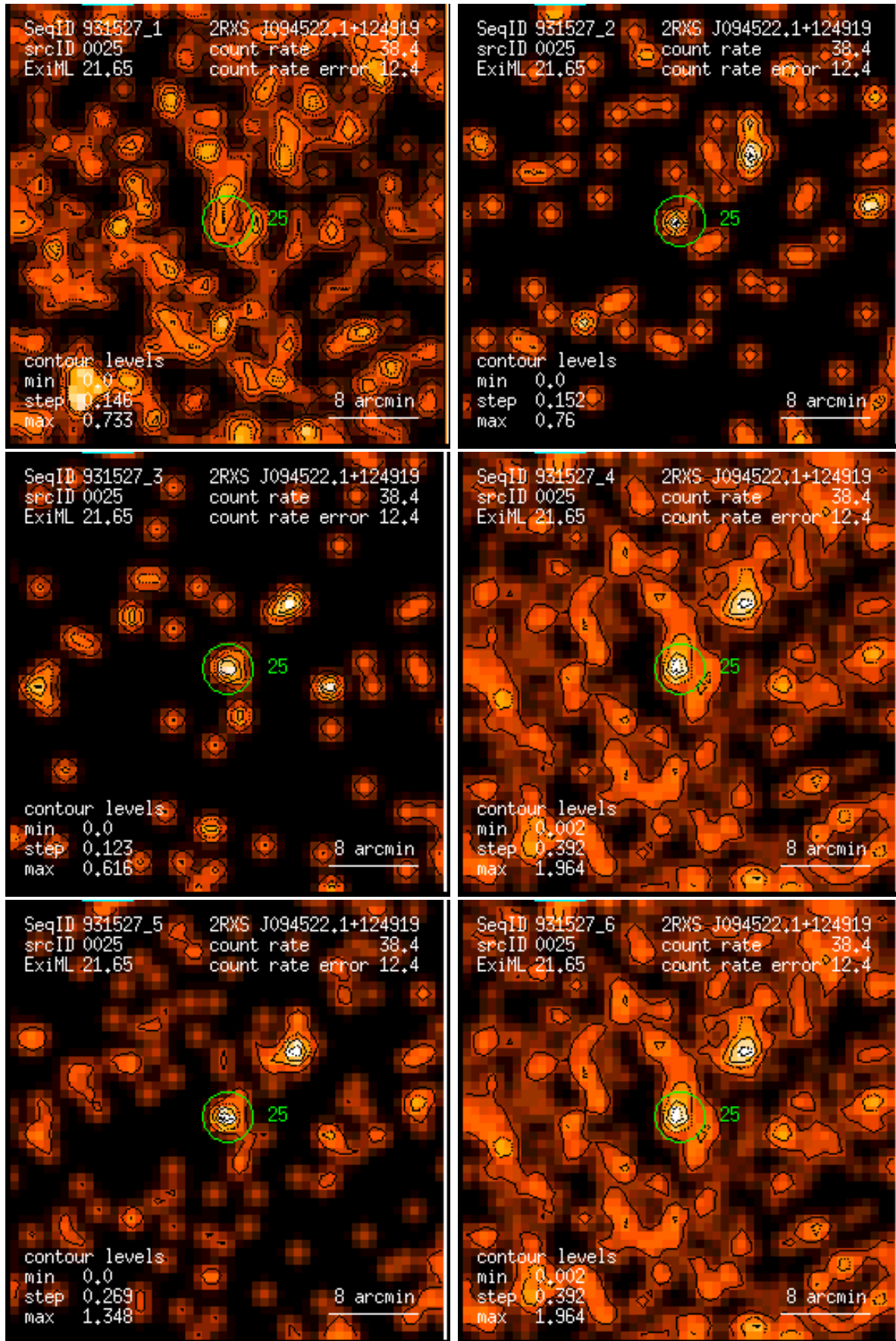
Figure 25: RASS 931527: detection 0025: band rate images, Gaussian filter: (1) PSPC channels 11 – 41, (2) 52 – 90, (3) 91 – 201, (4) 11 – 235, (5) 52 – 201, (6) 11 – 201. Broad band rates in counts/ks. Band rate contour levels in counts/ks/arcmin 2 .
