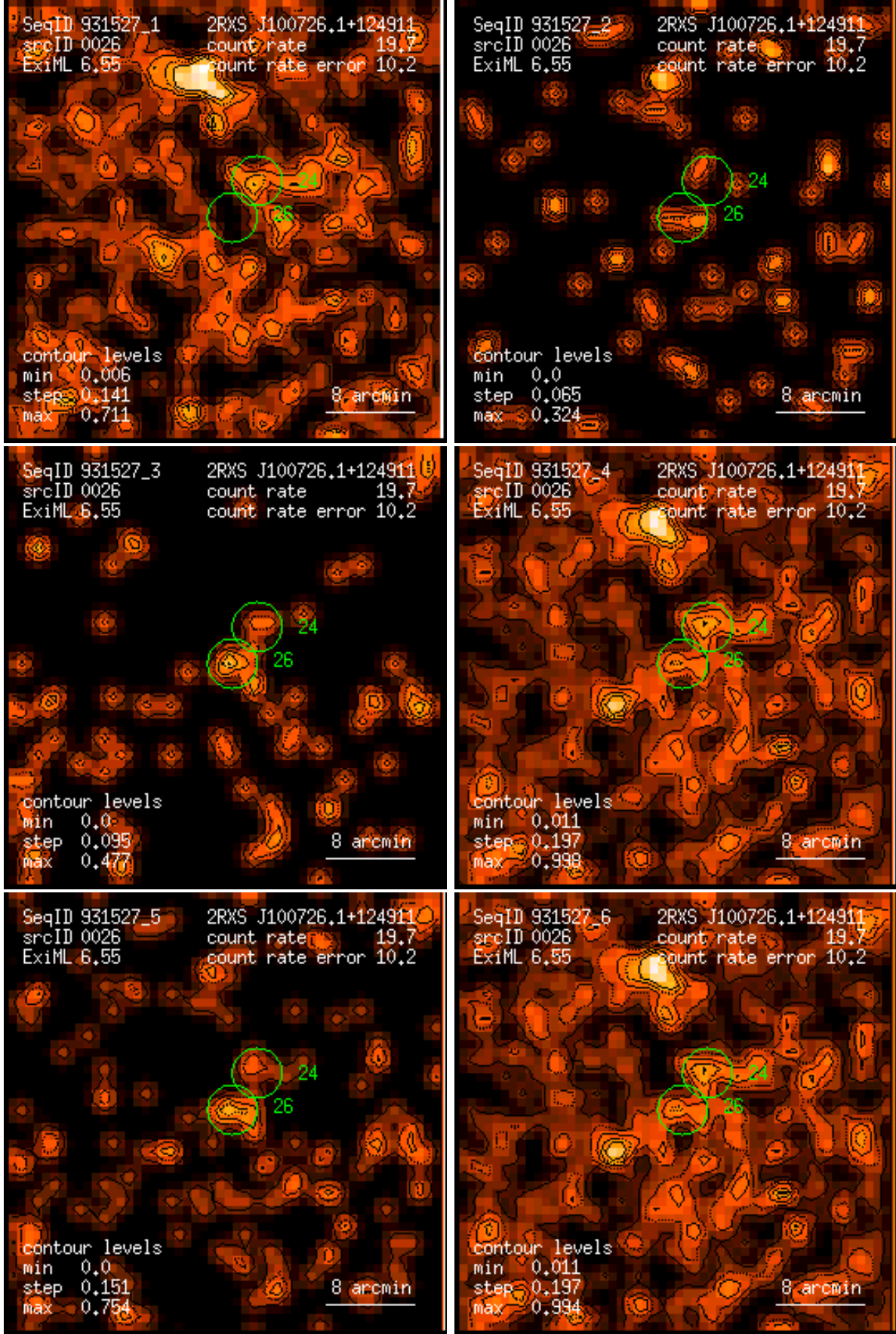
Figure 26: RASS 931527: detection 0026: band rate images, Gaussian filter: (1) PSPC channels 11 – 41, (2) 52 – 90, (3) 91 – 201, (4) 11 – 235, (5) 52 – 201, (6) 11 – 201. Broad band rates in counts/ks. Band rate contour levels in counts/ks/arcmin 2 .
