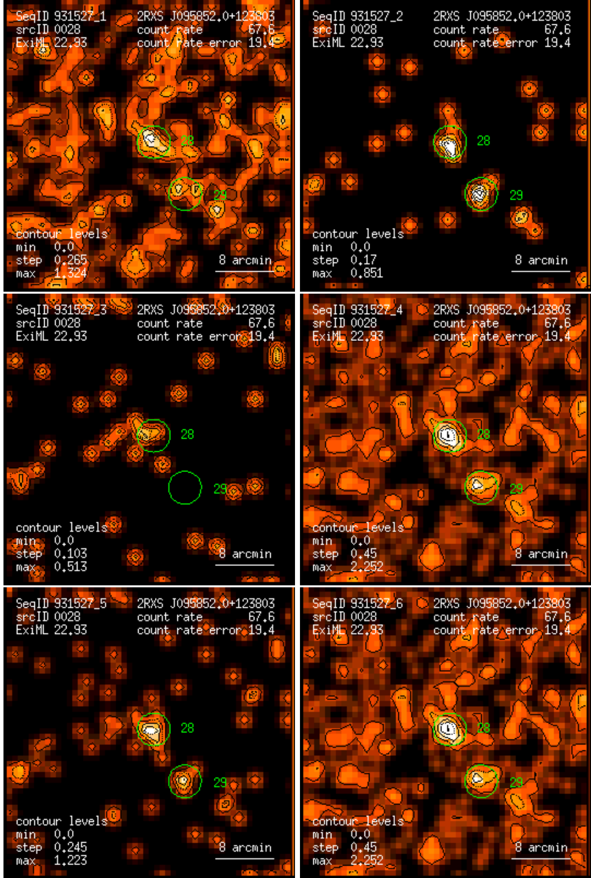
Figure 28: RASS 931527: detection 0028: band rate images, Gaussian filter: (1) PSPC channels 11 – 41, (2) 52 – 90, (3) 91 – 201, (4) 11 – 235, (5) 52 – 201, (6) 11 – 201. Broad band rates in counts/ks. Band rate contour levels in counts/ks/arcmin 2 .
