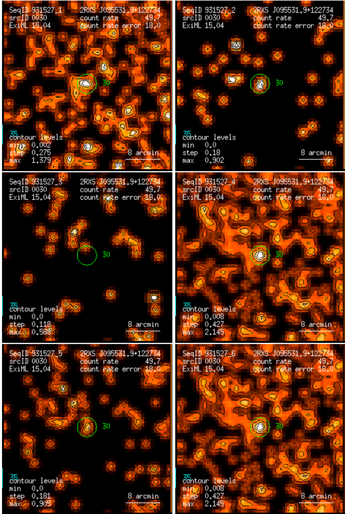
Figure 30: RASS 931527: detection 0030: band rate images, Gaussian filter: (1) PSPC channels 11 – 41, (2) 52 – 90, (3) 91 – 201, (4) 11 – 235, (5) 52 – 201, (6) 11 – 201. Broad band rates in counts/ks. Band rate contour levels in counts/ks/arcmin 2 .
