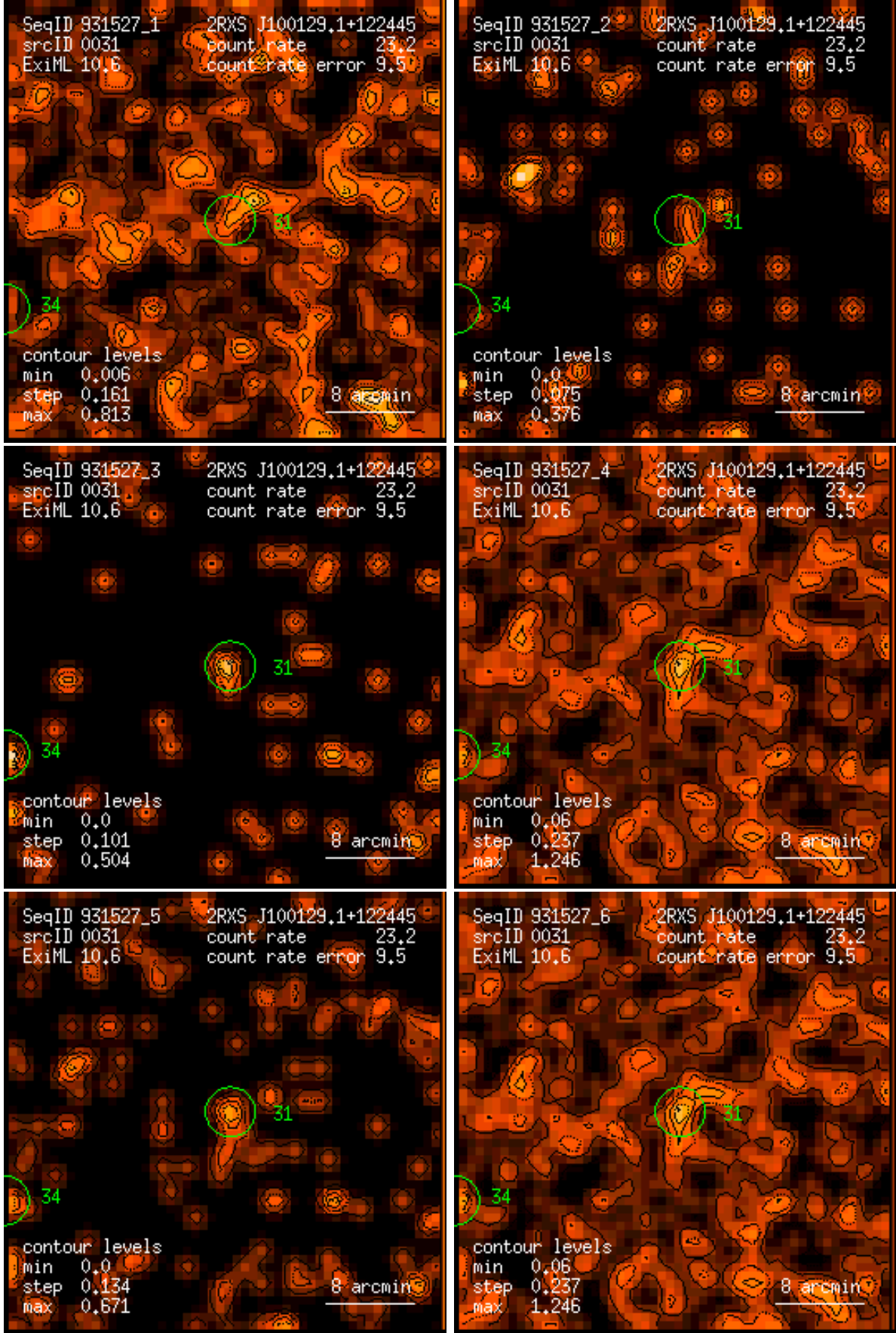
Figure 31: RASS 931527: detection 0031: band rate images, Gaussian filter: (1) PSPC channels 11 – 41, (2) 52 – 90, (3) 91 – 201, (4) 11 – 235, (5) 52 – 201, (6) 11 – 201. Broad band rates in counts/ks. Band rate contour levels in counts/ks/arcmin 2 .
