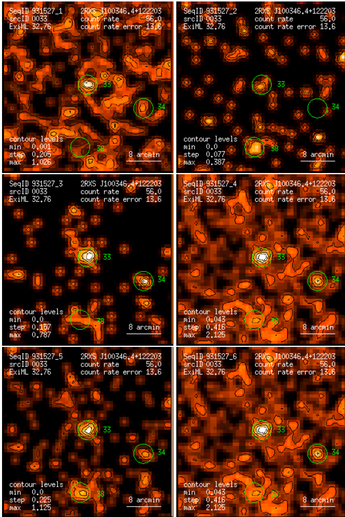
Figure 33: RASS 931527: detection 0033: band rate images, Gaussian filter: (1) PSPC channels 11 – 41, (2) 52 – 90, (3) 91 – 201, (4) 11 – 235, (5) 52 – 201, (6) 11 – 201. Broad band rates in counts/ks. Band rate contour levels in counts/ks/arcmin 2 .
