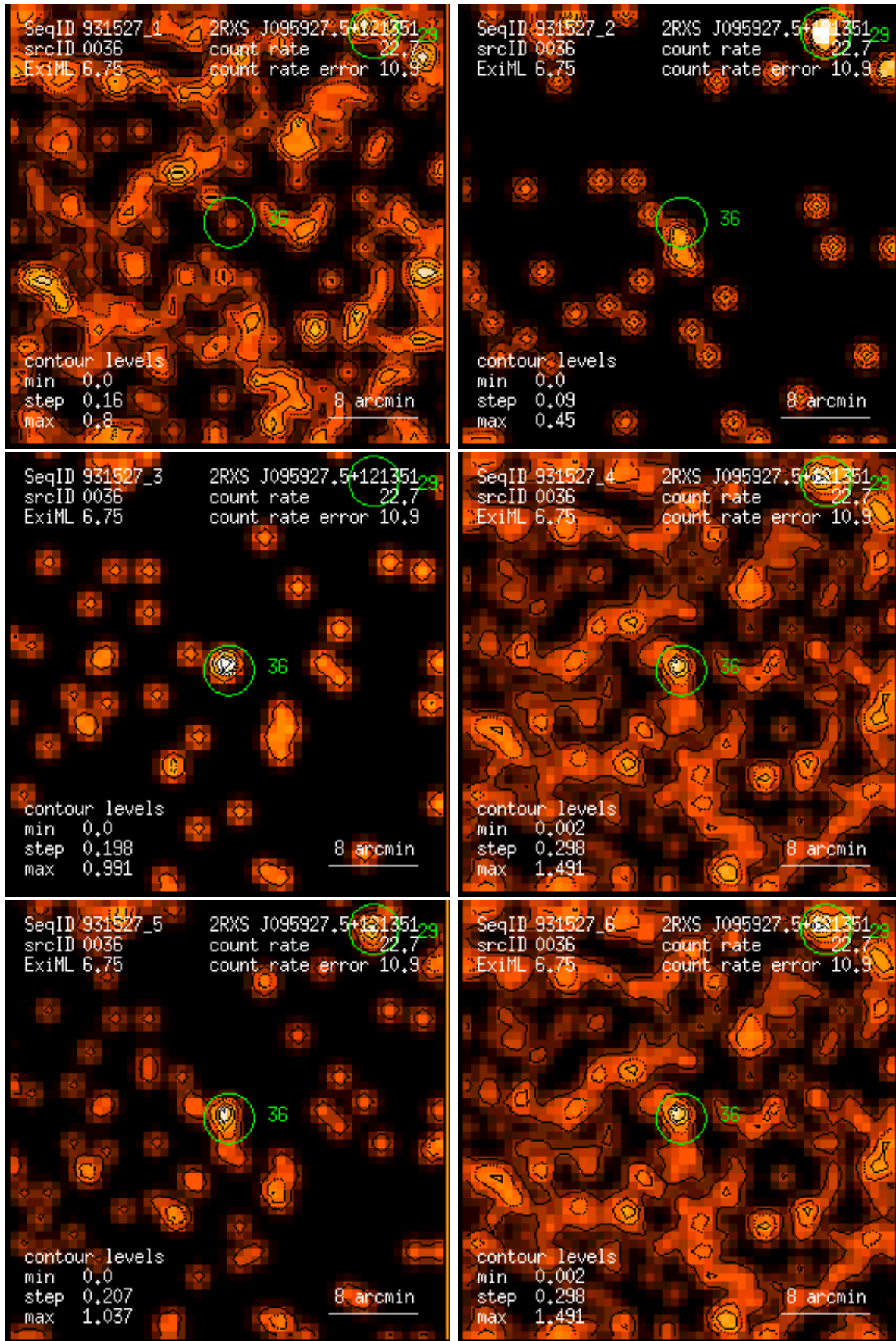
Figure 36: RASS 931527: detection 0036: band rate images, Gaussian filter: (1) PSPC channels 11 – 41, (2) 52 – 90, (3) 91 – 201, (4) 11 – 235, (5) 52 – 201, (6) 11 – 201. Broad band rates in counts/ks. Band rate contour levels in counts/ks/arcmin 2 .
