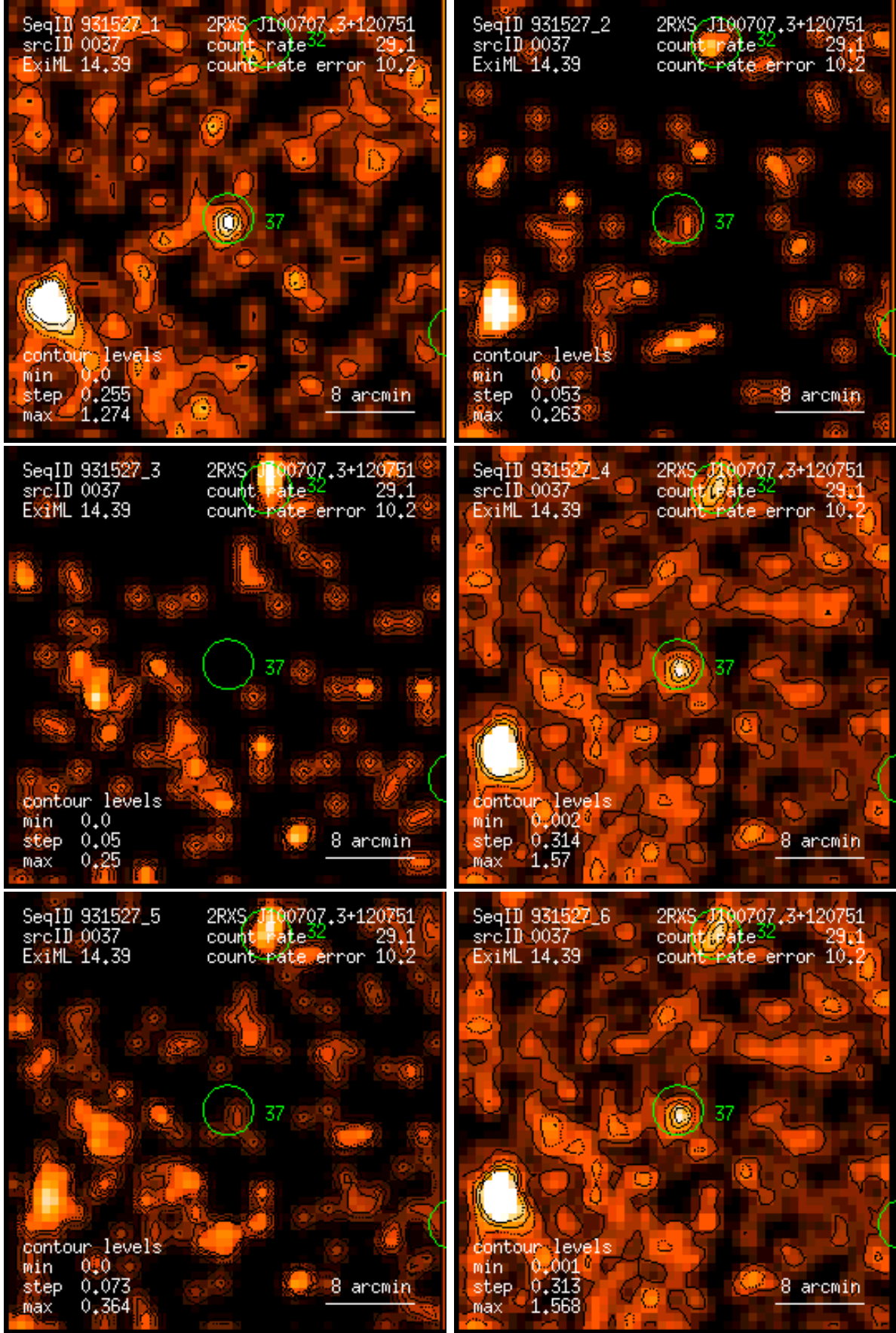
Figure 37: RASS 931527: detection 0037: band rate images, Gaussian filter: (1) PSPC channels 11 – 41, (2) 52 – 90, (3) 91 – 201, (4) 11 – 235, (5) 52 – 201, (6) 11 – 201. Broad band rates in counts/ks. Band rate contour levels in counts/ks/arcmin 2 .
