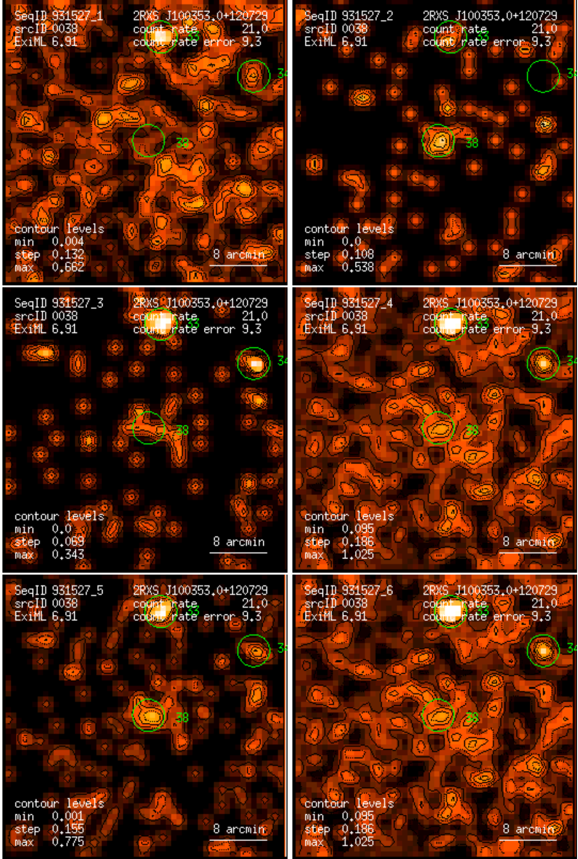
Figure 38: RASS 931527: detection 0038: band rate images, Gaussian filter: (1) PSPC channels 11 – 41, (2) 52 – 90, (3) 91 – 201, (4) 11 – 235, (5) 52 – 201, (6) 11 – 201. Broad band rates in counts/ks. Band rate contour levels in counts/ks/arcmin 2 .
