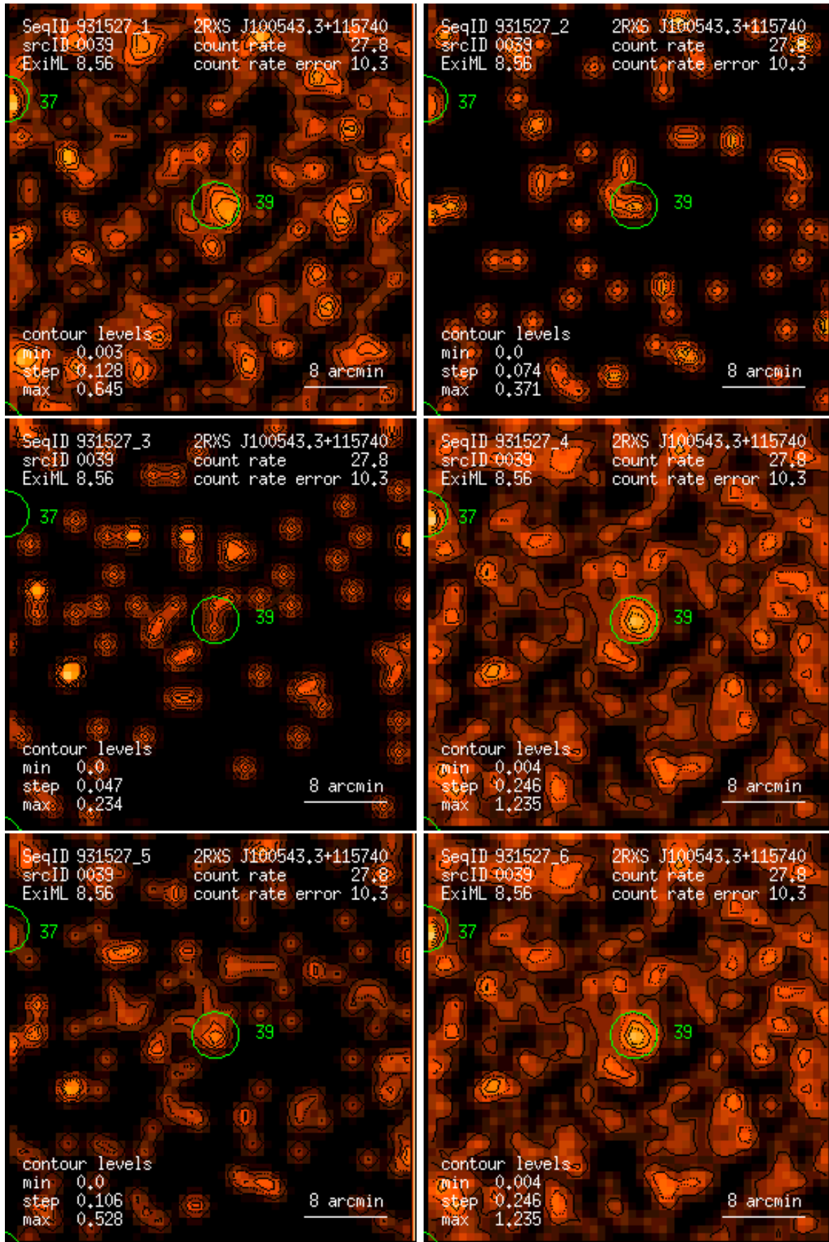
Figure 39: RASS 931527: detection 0039: band rate images, Gaussian filter: (1) PSPC channels 11 – 41, (2) 52 – 90, (3) 91 – 201, (4) 11 – 235, (5) 52 – 201, (6) 11 – 201. Broad band rates in counts/ks. Band rate contour levels in counts/ks/arcmin 2 .
