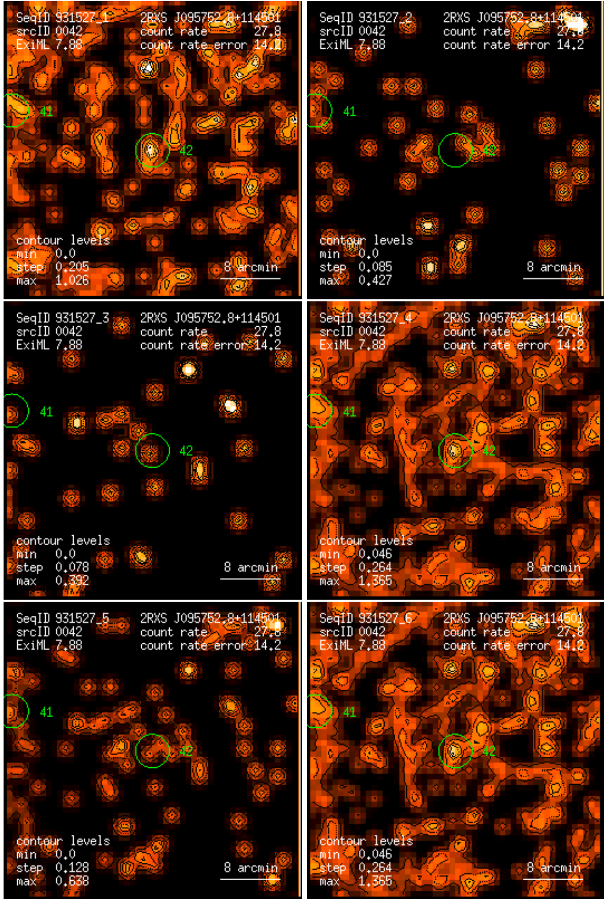
Figure 42: RASS 931527: detection 0042: band rate images, Gaussian filter: (1) PSPC channels 11 – 41, (2) 52 – 90, (3) 91 – 201, (4) 11 – 235, (5) 52 – 201, (6) 11 – 201. Broad band rates in counts/ks. Band rate contour levels in counts/ks/arcmin 2 .
