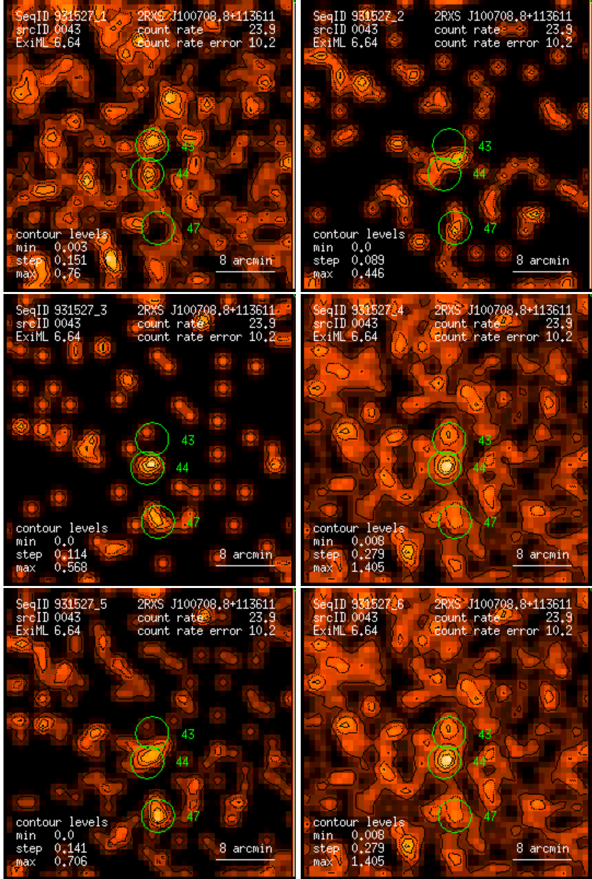
Figure 43: RASS 931527: detection 0043: band rate images, Gaussian filter: (1) PSPC channels 11 – 41, (2) 52 – 90, (3) 91 – 201, (4) 11 – 235, (5) 52 – 201, (6) 11 – 201. Broad band rates in counts/ks. Band rate contour levels in counts/ks/arcmin 2 .
