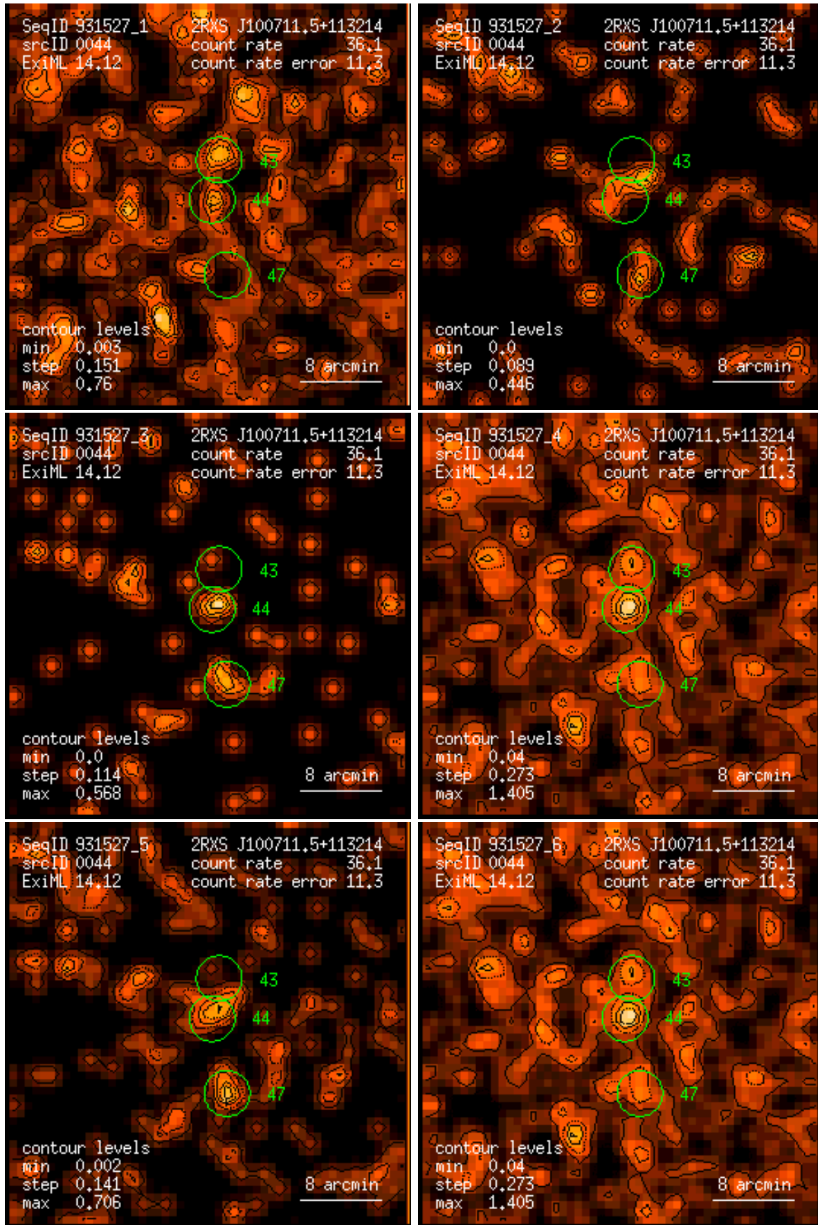
Figure 44: RASS 931527: detection 0044: band rate images, Gaussian filter: (1) PSPC channels 11 – 41, (2) 52 – 90, (3) 91 – 201, (4) 11 – 235, (5) 52 – 201, (6) 11 – 201. Broad band rates in counts/ks. Band rate contour levels in counts/ks/arcmin 2 .
