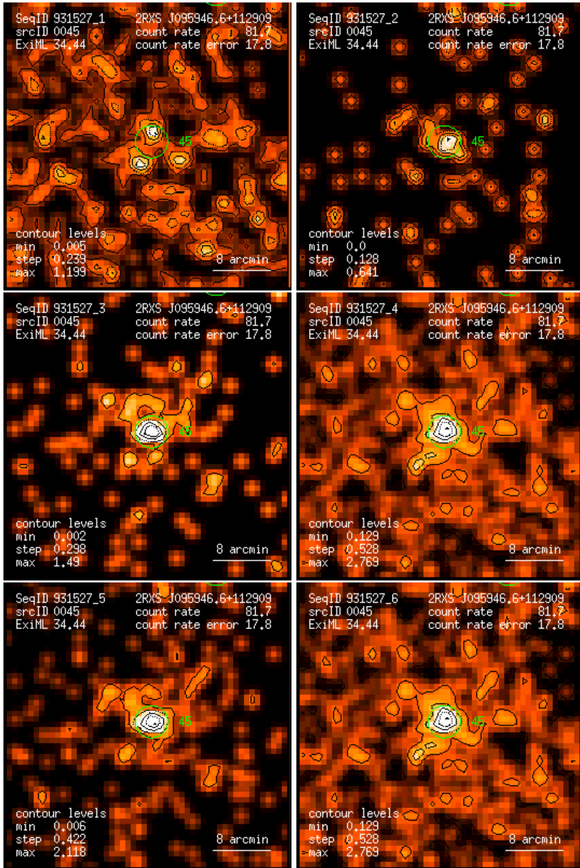
Figure 45: RASS 931527: detection 0045: band rate images, Gaussian filter: (1) PSPC channels 11 – 41, (2) 52 – 90, (3) 91 – 201, (4) 11 – 235, (5) 52 – 201, (6) 11 – 201. Broad band rates in counts/ks. Band rate contour levels in counts/ks/arcmin 2 .
