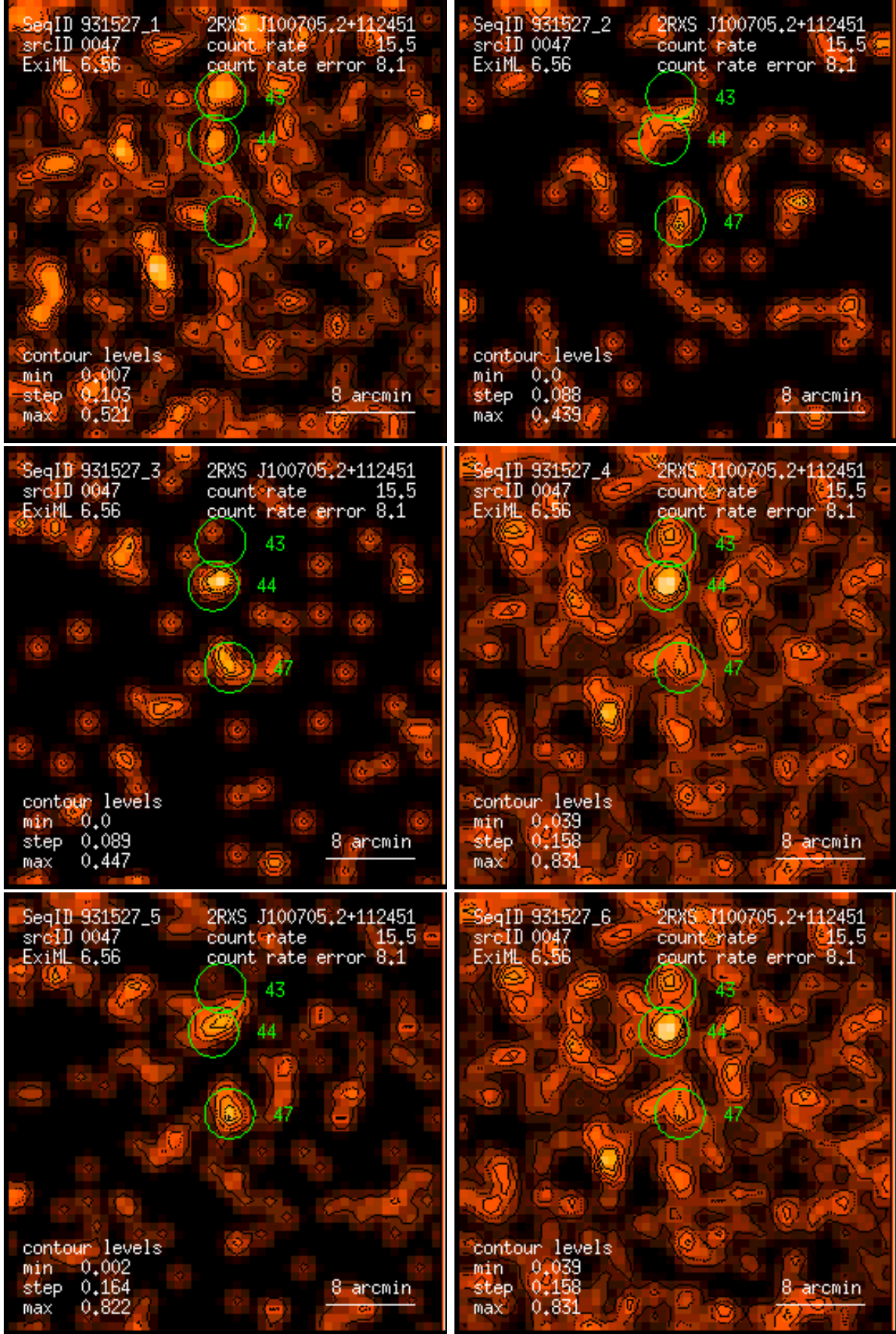
Figure 47: RASS 931527: detection 0047: band rate images, Gaussian filter: (1) PSPC channels 11 – 41, (2) 52 – 90, (3) 91 – 201, (4) 11 – 235, (5) 52 – 201, (6) 11 – 201. Broad band rates in counts/ks. Band rate contour levels in counts/ks/arcmin 2 .
