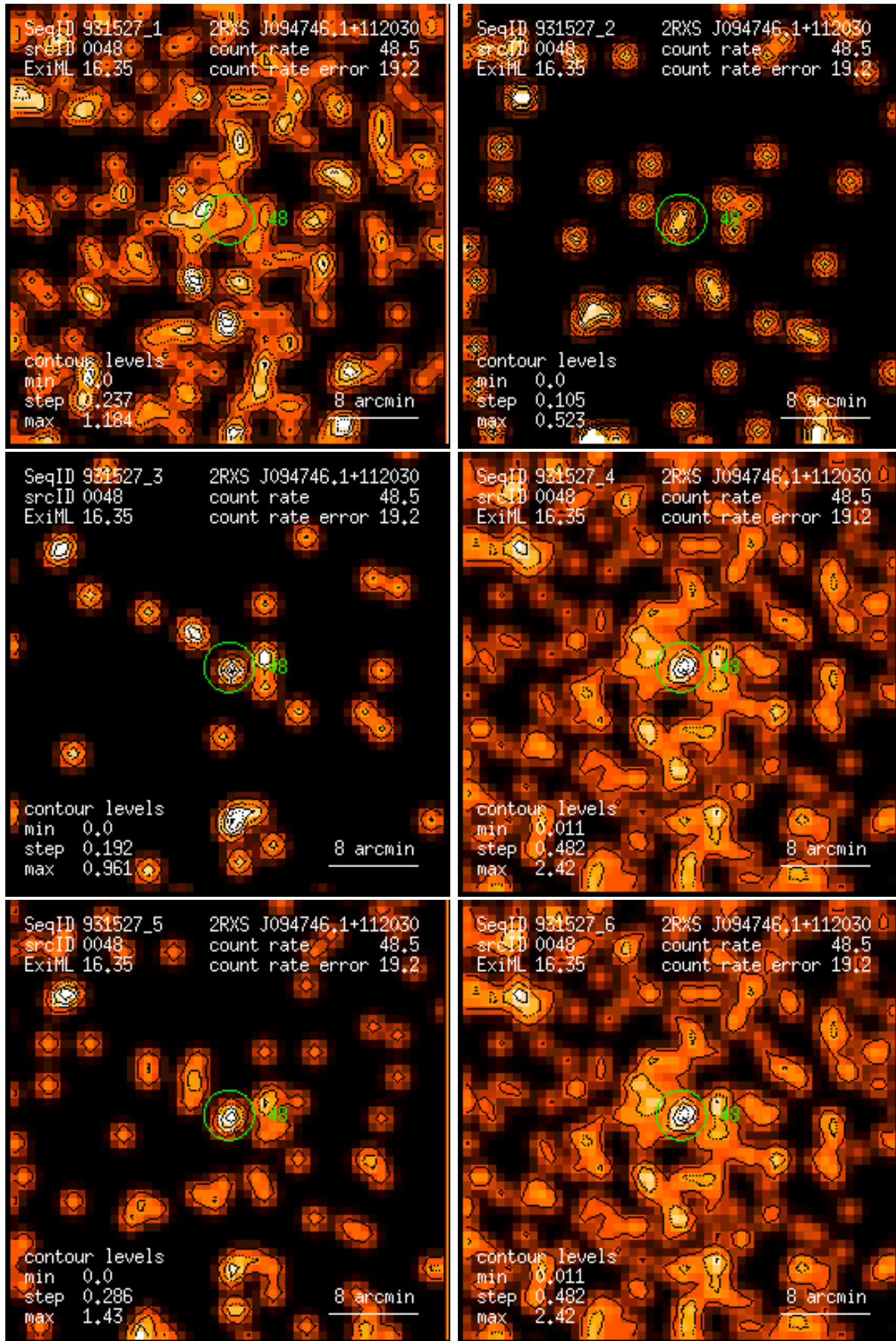
Figure 48: RASS 931527: detection 0048: band rate images, Gaussian filter: (1) PSPC channels 11 – 41, (2) 52 – 90, (3) 91 – 201, (4) 11 – 235, (5) 52 – 201, (6) 11 – 201. Broad band rates in counts/ks. Band rate contour levels in counts/ks/arcmin 2 .
