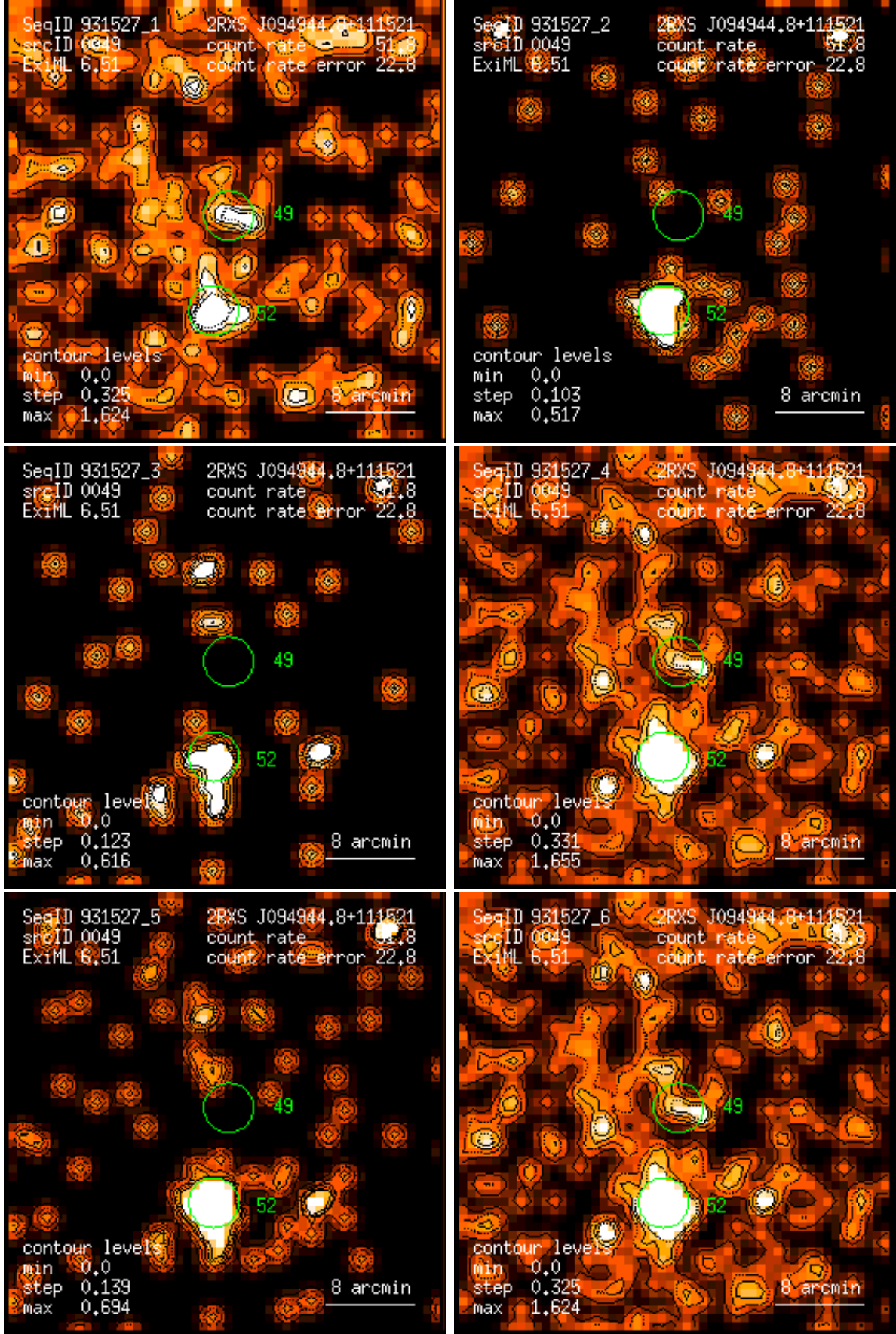
Figure 49: RASS 931527: detection 0049: band rate images, Gaussian filter: (1) PSPC channels 11 – 41, (2) 52 – 90, (3) 91 – 201, (4) 11 – 235, (5) 52 – 201, (6) 11 – 201. Broad band rates in counts/ks. Band rate contour levels in counts/ks/arcmin 2 .
