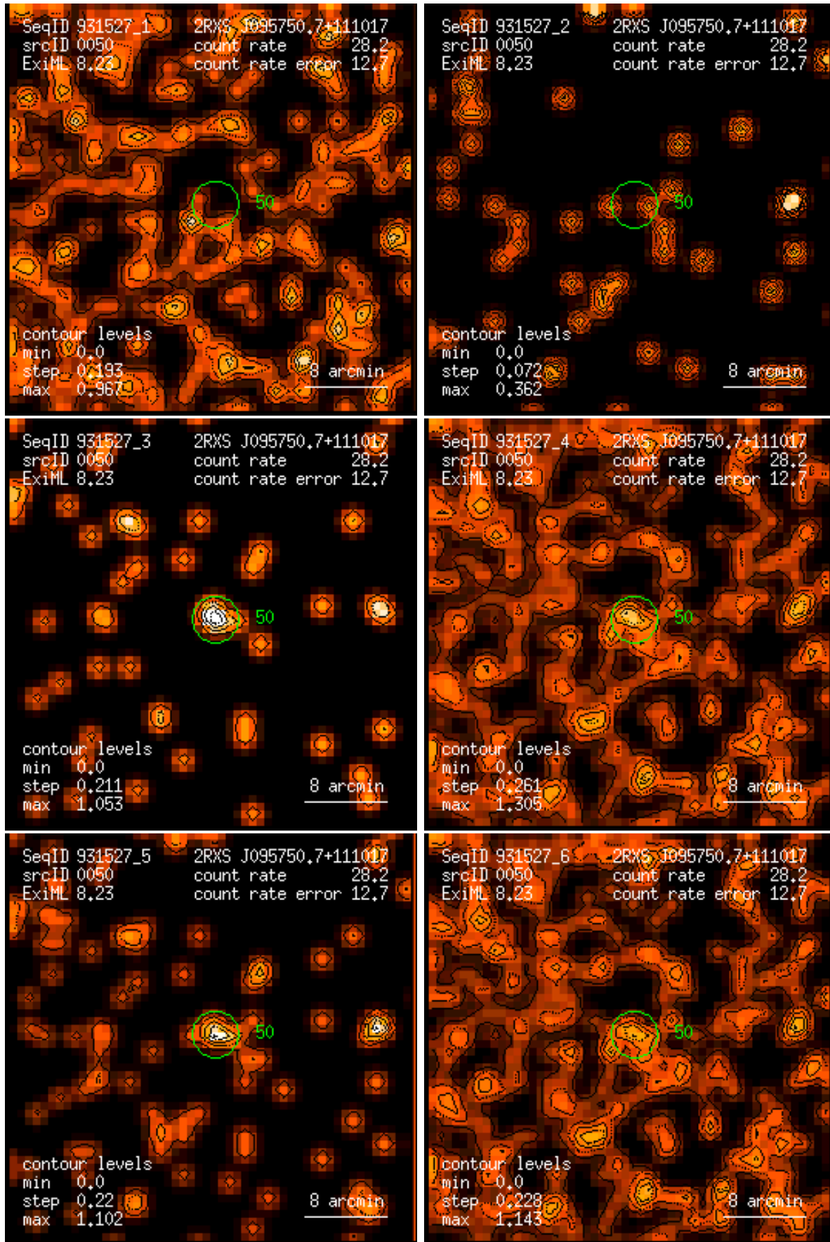
Figure 50: RASS 931527: detection 0050: band rate images, Gaussian filter: (1) PSPC channels 11 – 41, (2) 52 – 90, (3) 91 – 201, (4) 11 – 235, (5) 52 – 201, (6) 11 – 201. Broad band rates in counts/ks. Band rate contour levels in counts/ks/arcmin 2 .
