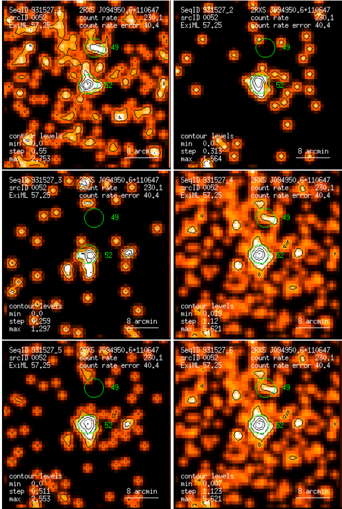
Figure 52: RASS 931527: detection 0052: band rate images, Gaussian filter: (1) PSPC channels 11 – 41, (2) 52 – 90, (3) 91 – 201, (4) 11 – 235, (5) 52 – 201, (6) 11 – 201. Broad band rates in counts/ks. Band rate contour levels in counts/ks/arcmin 2 .
