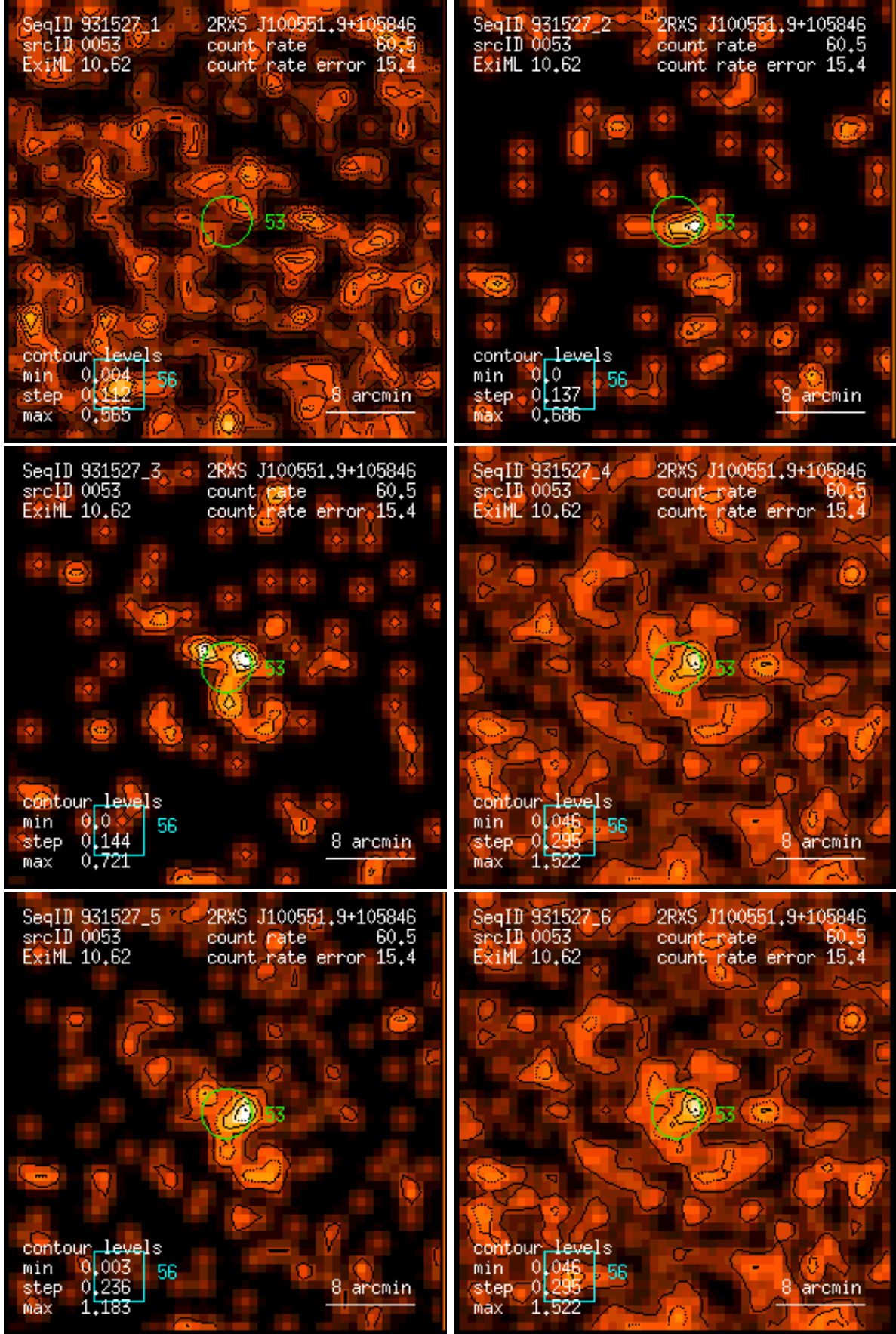
Figure 53: RASS 931527: detection 0053: band rate images, Gaussian filter: (1) PSPC channels 11 – 41, (2) 52 – 90, (3) 91 – 201, (4) 11 – 235, (5) 52 – 201, (6) 11 – 201. Broad band rates in counts/ks. Band rate contour levels in counts/ks/arcmin 2 .
