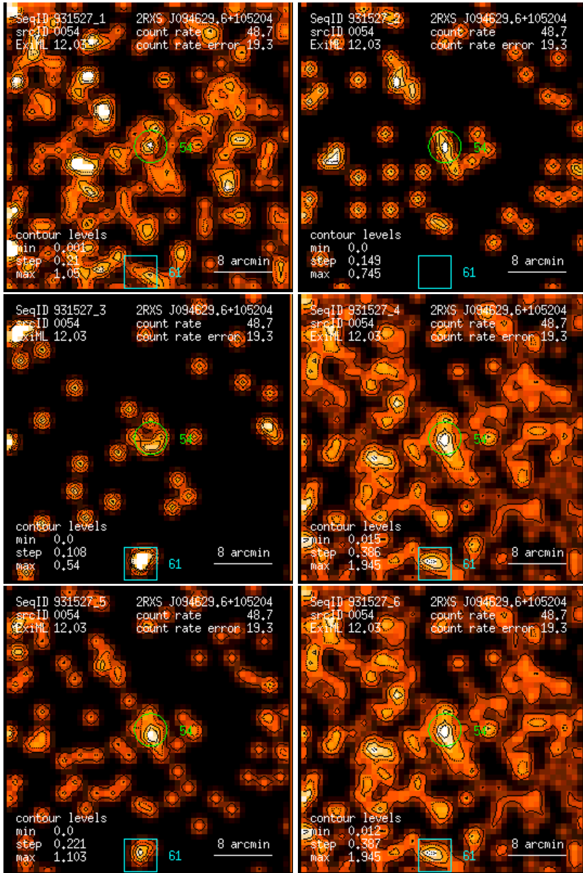
Figure 54: RASS 931527: detection 0054: band rate images, Gaussian filter: (1) PSPC channels 11 – 41, (2) 52 – 90, (3) 91 – 201, (4) 11 – 235, (5) 52 – 201, (6) 11 – 201. Broad band rates in counts/ks. Band rate contour levels in counts/ks/arcmin 2 .
