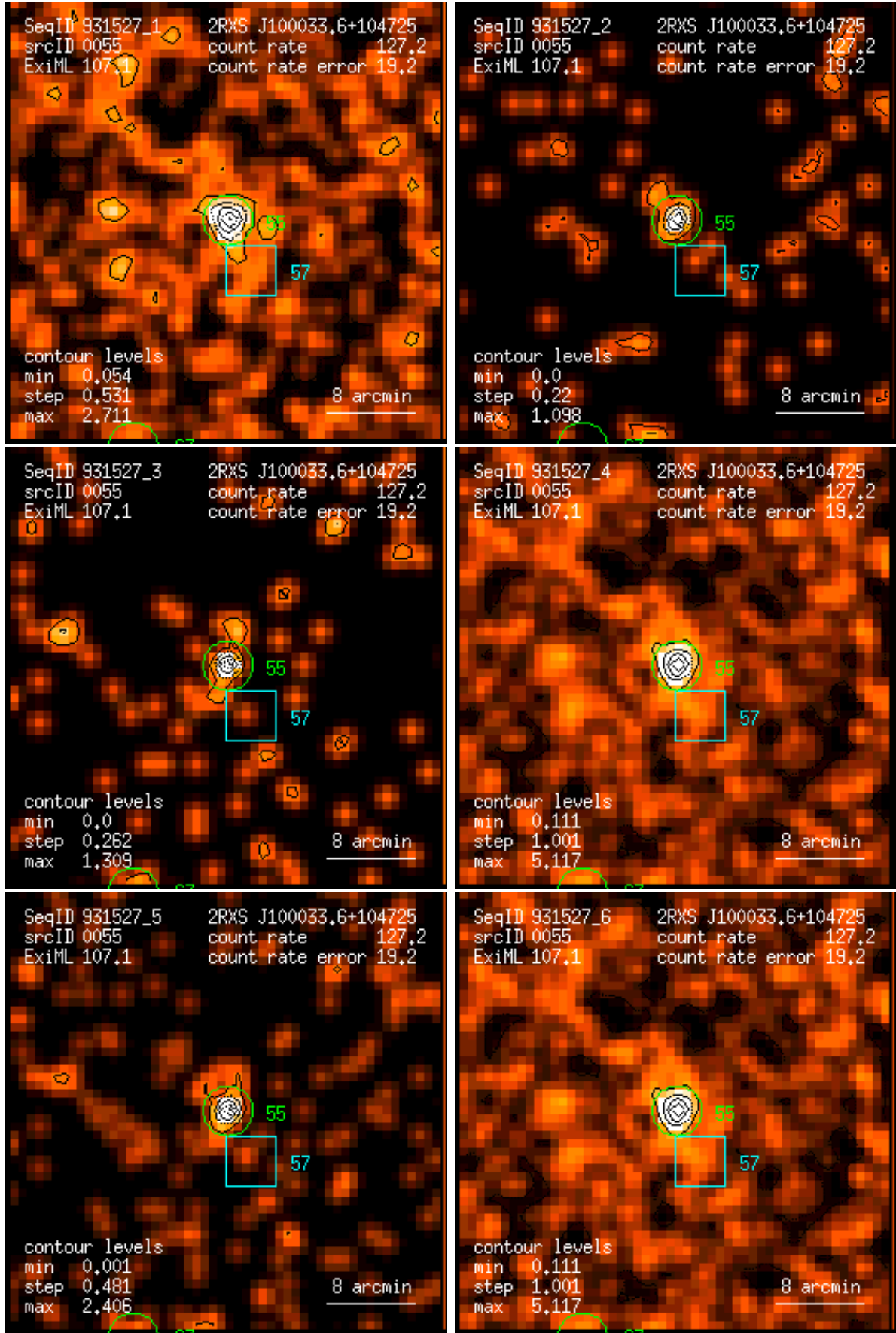
Figure 55: RASS 931527: detection 0055: band rate images, Gaussian filter: (1) PSPC channels 11 – 41, (2) 52 – 90, (3) 91 – 201, (4) 11 – 235, (5) 52 – 201, (6) 11 – 201. Broad band rates in counts/ks. Band rate contour levels in counts/ks/arcmin 2 .
