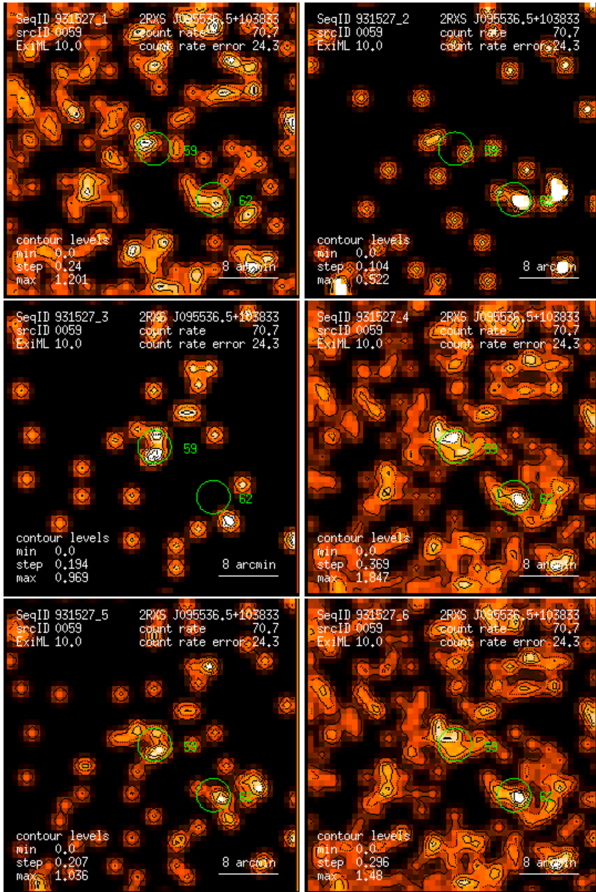
Figure 59: RASS 931527: detection 0059: band rate images, Gaussian filter: (1) PSPC channels 11 – 41, (2) 52 – 90, (3) 91 – 201, (4) 11 – 235, (5) 52 – 201, (6) 11 – 201. Broad band rates in counts/ks. Band rate contour levels in counts/ks/arcmin 2 .
