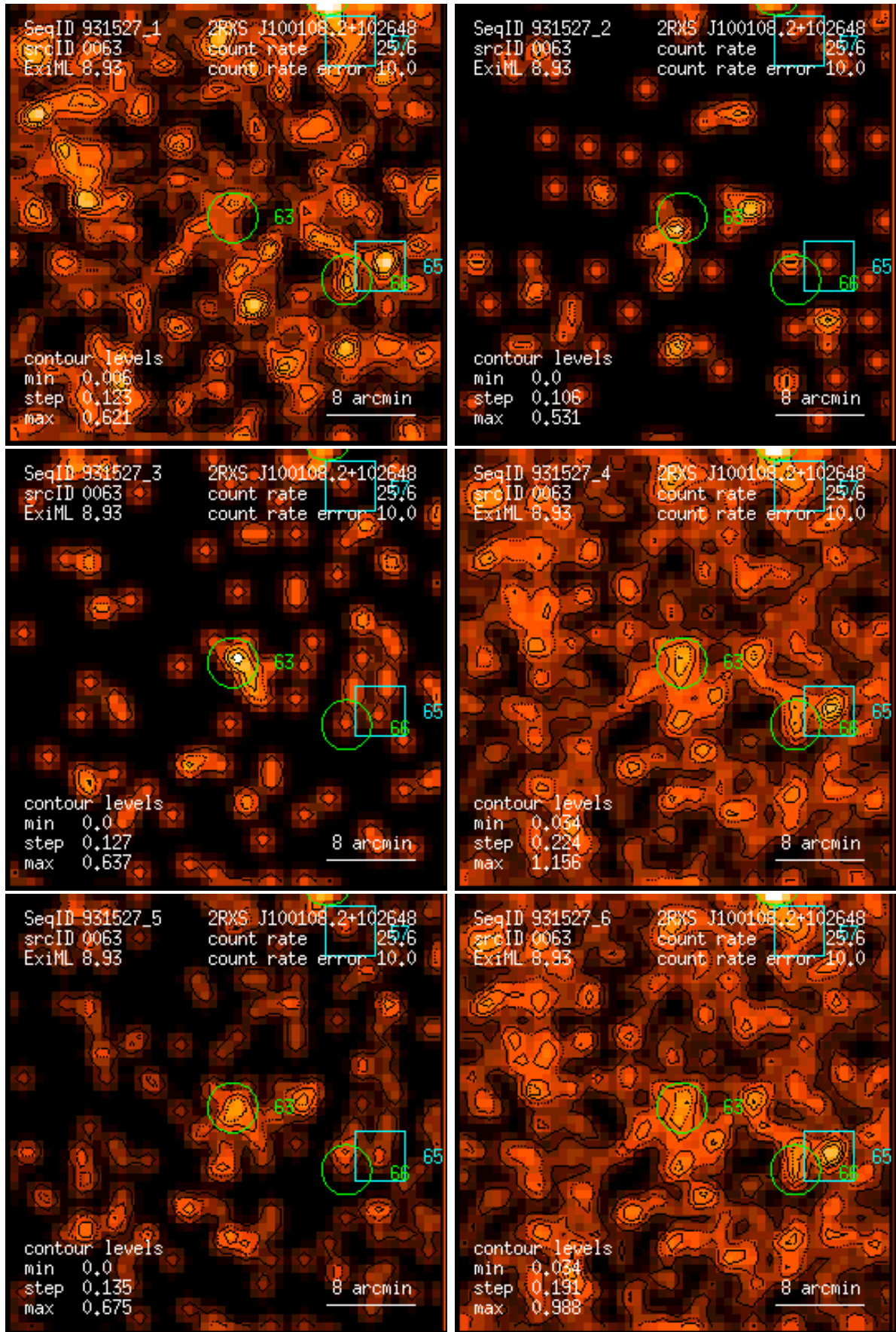
Figure 63: RASS 931527: detection 0063: band rate images, Gaussian filter: (1) PSPC channels 11 – 41, (2) 52 – 90, (3) 91 – 201, (4) 11 – 235, (5) 52 – 201, (6) 11 – 201. Broad band rates in counts/ks. Band rate contour levels in counts/ks/arcmin 2 .
