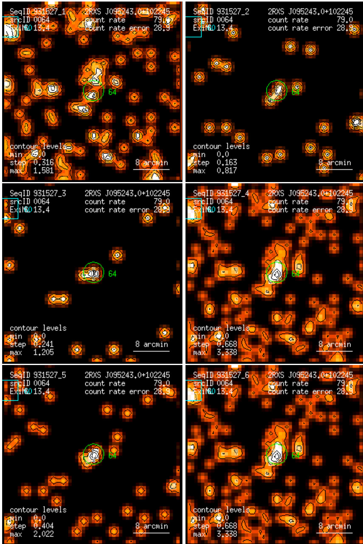
Figure 64: RASS 931527: detection 0064: band rate images, Gaussian filter: (1) PSPC channels 11 – 41, (2) 52 – 90, (3) 91 – 201, (4) 11 – 235, (5) 52 – 201, (6) 11 – 201. Broad band rates in counts/ks. Band rate contour levels in counts/ks/arcmin 2 .
