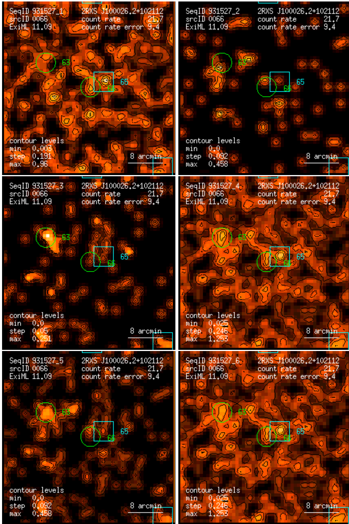
Figure 66: RASS 931527: detection 0066: band rate images, Gaussian filter: (1) PSPC channels 11 – 41, (2) 52 – 90, (3) 91 – 201, (4) 11 – 235, (5) 52 – 201, (6) 11 – 201. Broad band rates in counts/ks. Band rate contour levels in counts/ks/arcmin 2 .
