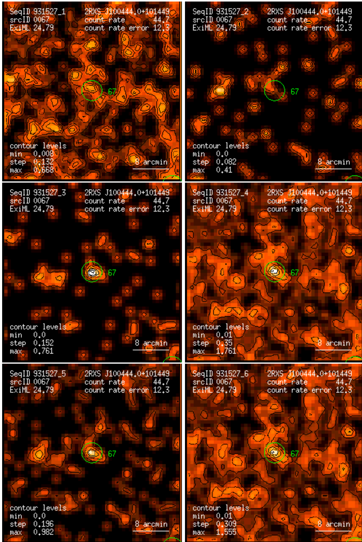
Figure 67: RASS 931527: detection 0067: band rate images, Gaussian filter: (1) PSPC channels 11 – 41, (2) 52 – 90, (3) 91 – 201, (4) 11 – 235, (5) 52 – 201, (6) 11 – 201. Broad band rates in counts/ks. Band rate contour levels in counts/ks/arcmin 2 .
