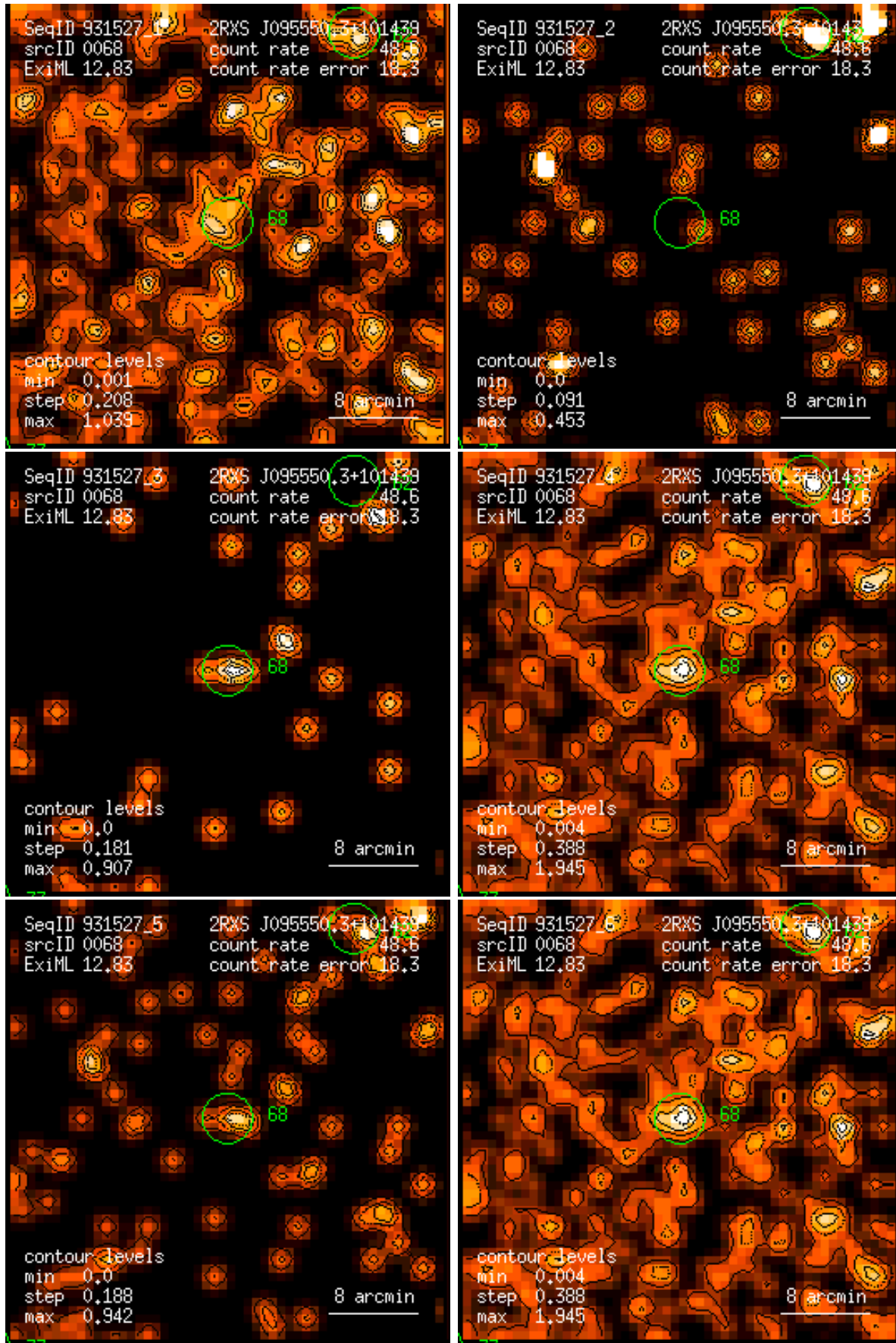
Figure 68: RASS 931527: detection 0068: band rate images, Gaussian filter: (1) PSPC channels 11 – 41, (2) 52 – 90, (3) 91 – 201, (4) 11 – 235, (5) 52 – 201, (6) 11 – 201. Broad band rates in counts/ks. Band rate contour levels in counts/ks/arcmin 2 .
