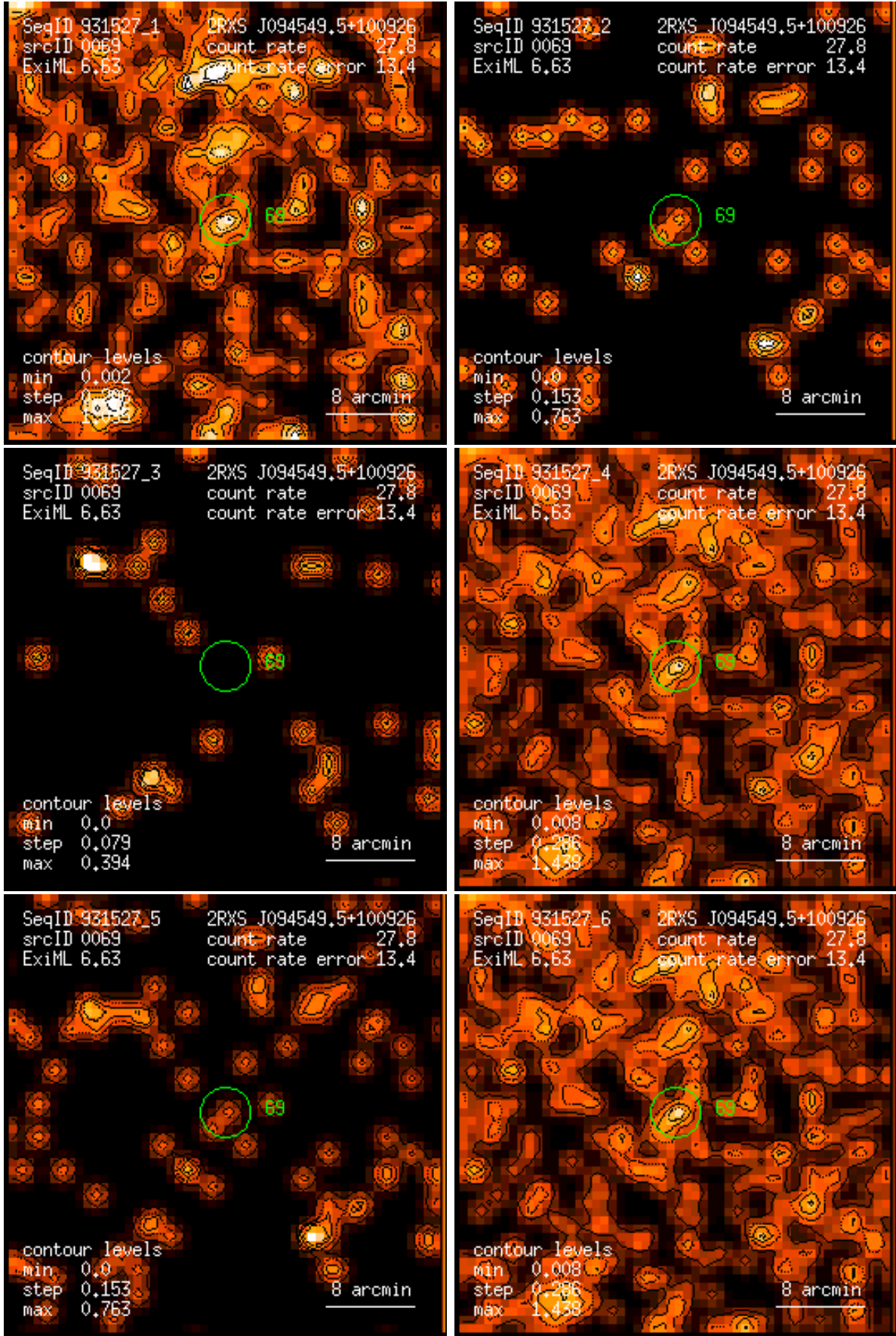
Figure 69: RASS 931527: detection 0069: band rate images, Gaussian filter: (1) PSPC channels 11 – 41, (2) 52 – 90, (3) 91 – 201, (4) 11 – 235, (5) 52 – 201, (6) 11 – 201. Broad band rates in counts/ks. Band rate contour levels in counts/ks/arcmin 2 .
