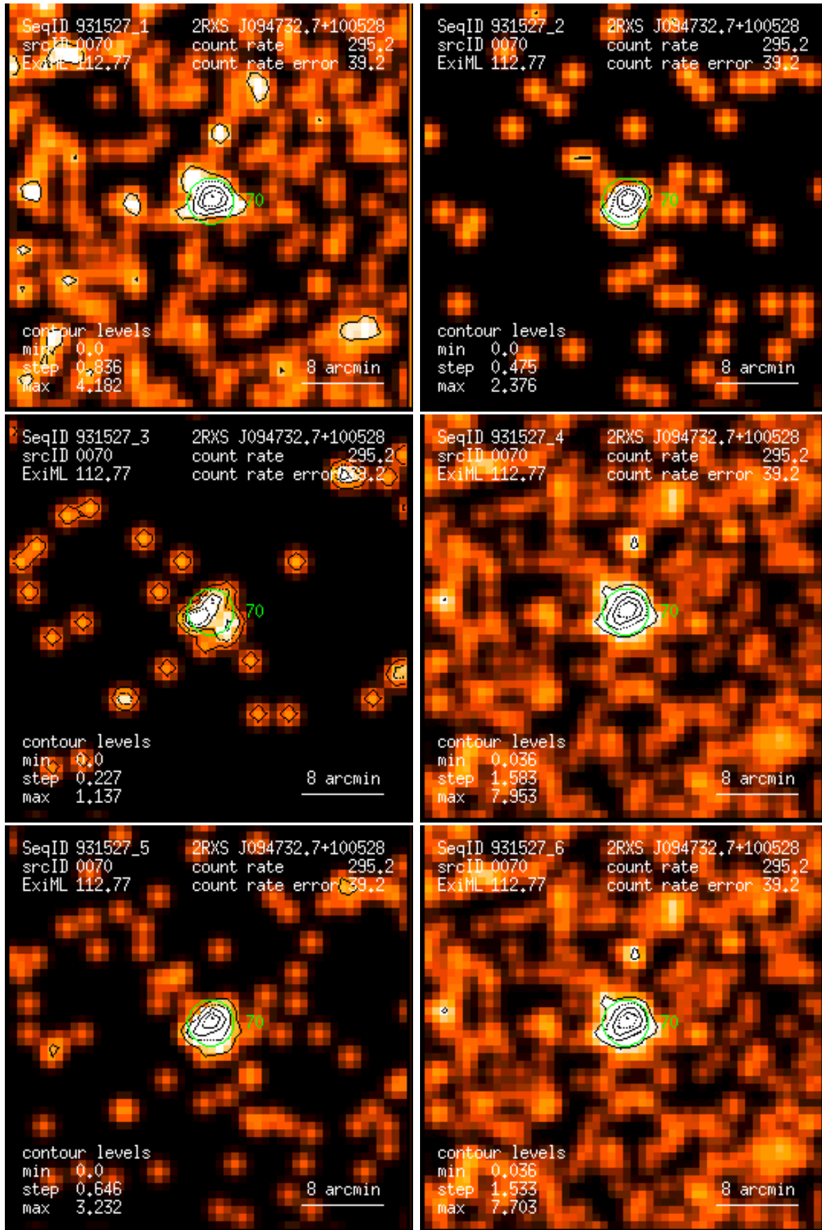
Figure 70: RASS 931527: detection 0070: band rate images, Gaussian filter: (1) PSPC channels 11 – 41, (2) 52 – 90, (3) 91 – 201, (4) 11 – 235, (5) 52 – 201, (6) 11 – 201. Broad band rates in counts/ks. Band rate contour levels in counts/ks/arcmin 2 .
