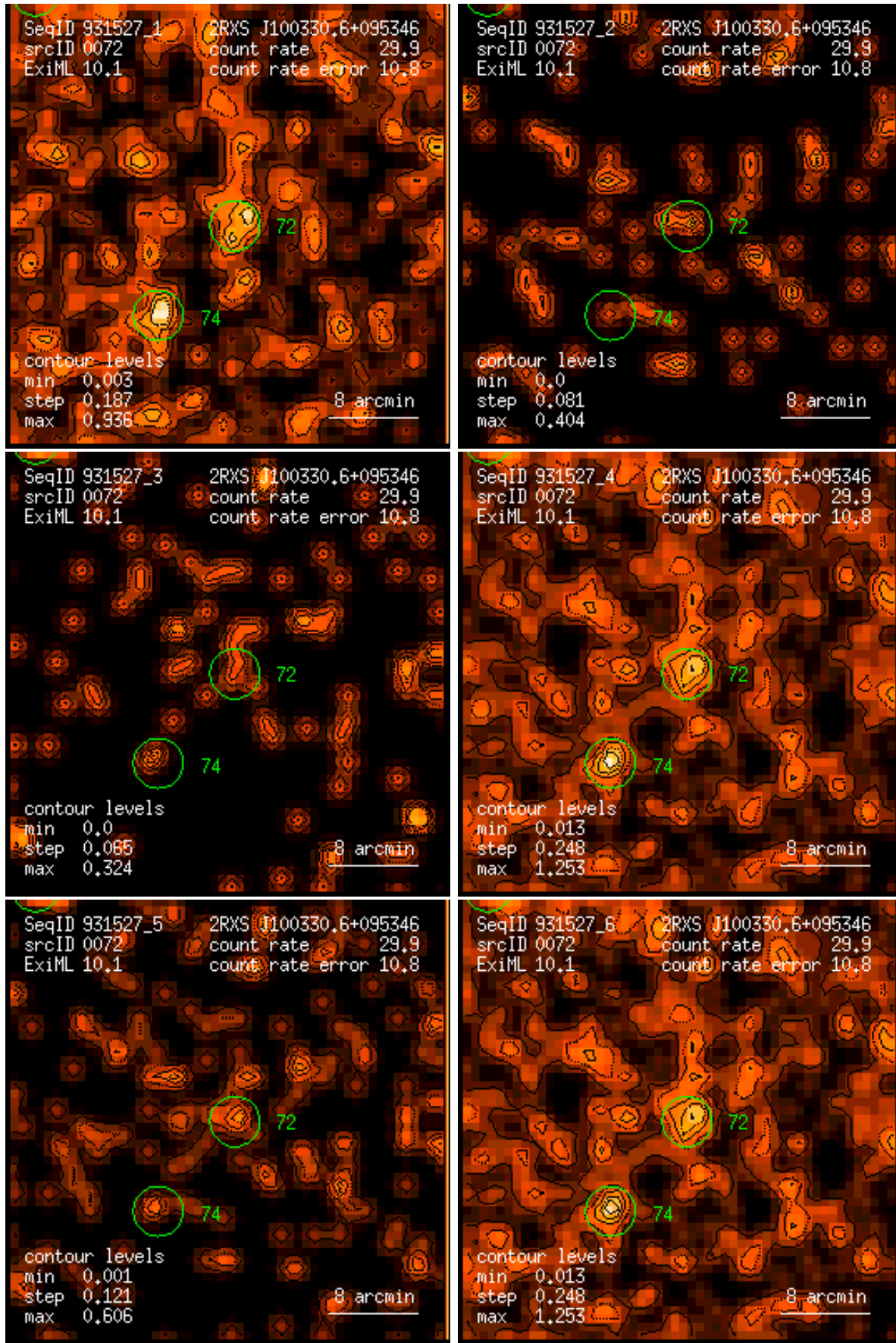
Figure 72: RASS 931527: detection 0072: band rate images, Gaussian filter: (1) PSPC channels 11 – 41, (2) 52 – 90, (3) 91 – 201, (4) 11 – 235, (5) 52 – 201, (6) 11 – 201. Broad band rates in counts/ks. Band rate contour levels in counts/ks/arcmin 2 .
