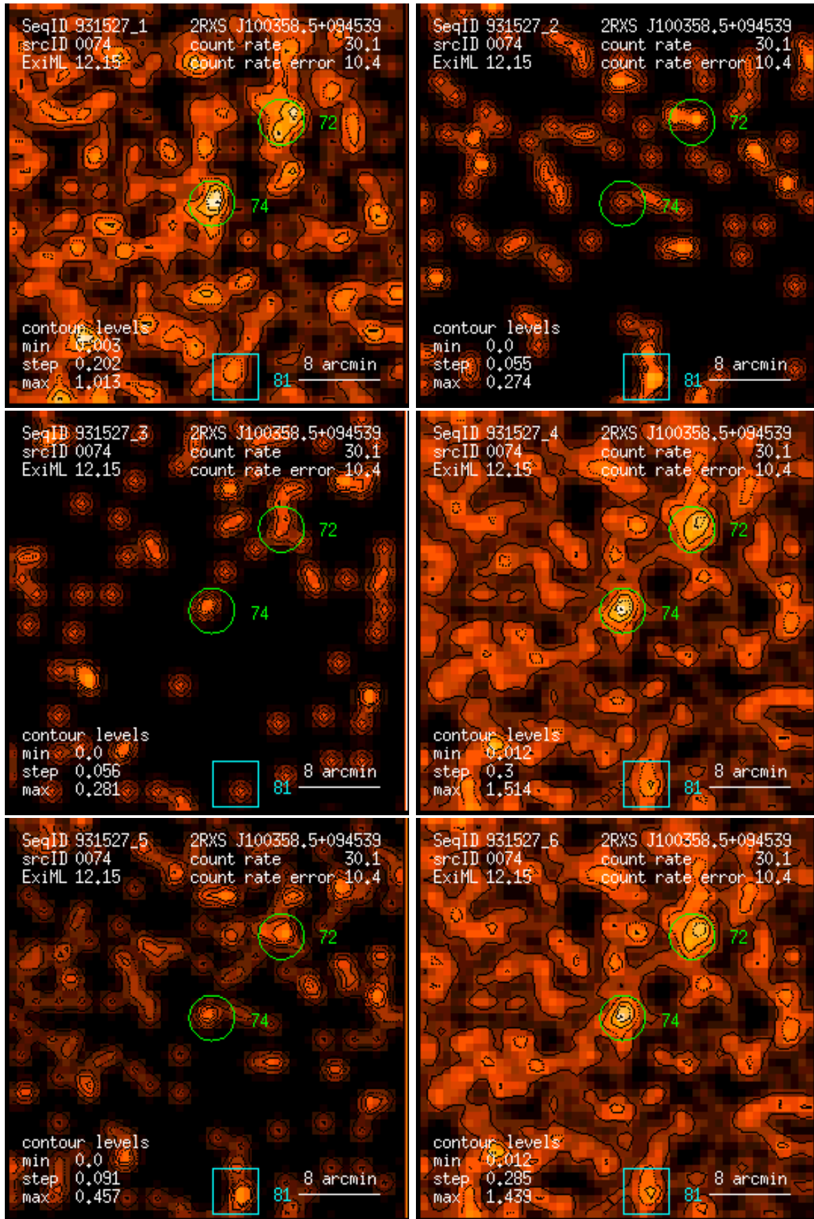
Figure 74: RASS 931527: detection 0074: band rate images, Gaussian filter: (1) PSPC channels 11 – 41, (2) 52 – 90, (3) 91 – 201, (4) 11 – 235, (5) 52 – 201, (6) 11 – 201. Broad band rates in counts/ks. Band rate contour levels in counts/ks/arcmin 2 .
