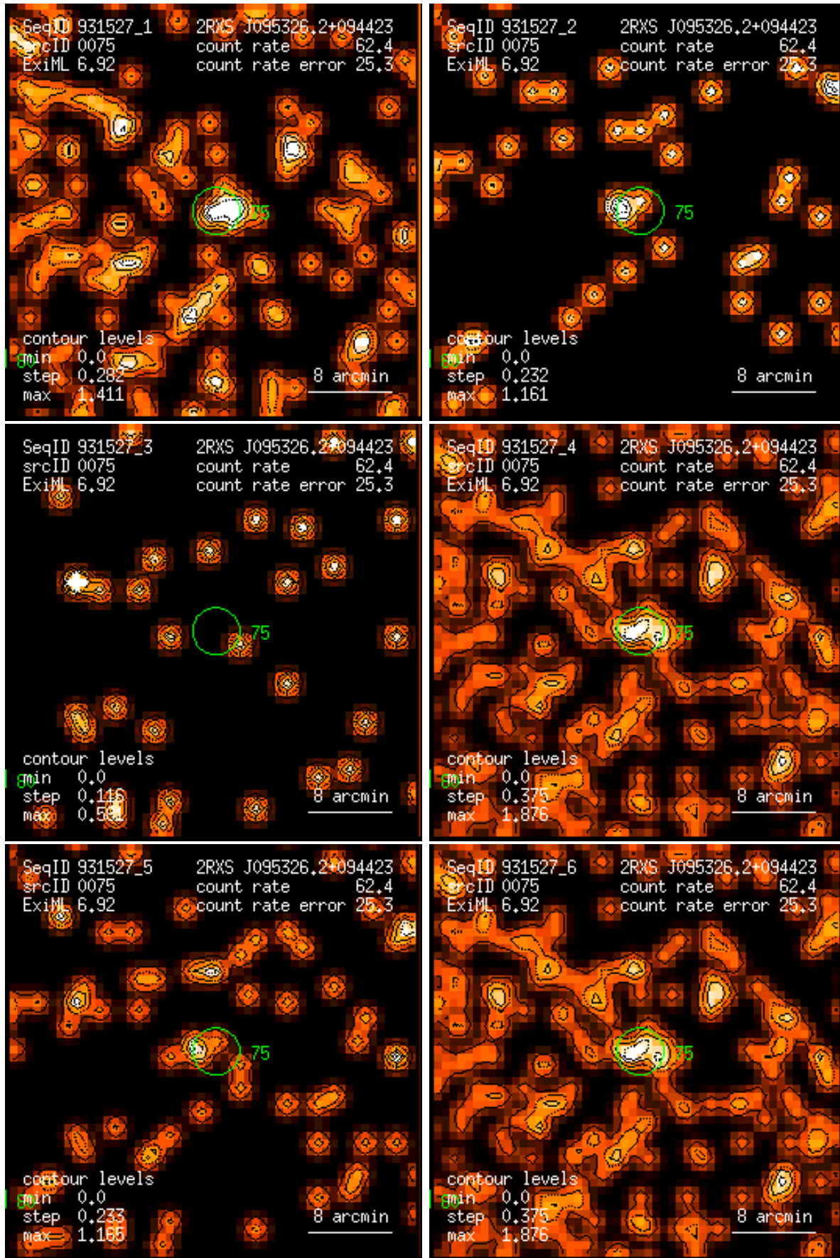
Figure 75: RASS 931527: detection 0075: band rate images, Gaussian filter: (1) PSPC channels 11 – 41, (2) 52 – 90, (3) 91 – 201, (4) 11 – 235, (5) 52 – 201, (6) 11 – 201. Broad band rates in counts/ks. Band rate contour levels in counts/ks/arcmin 2 .
