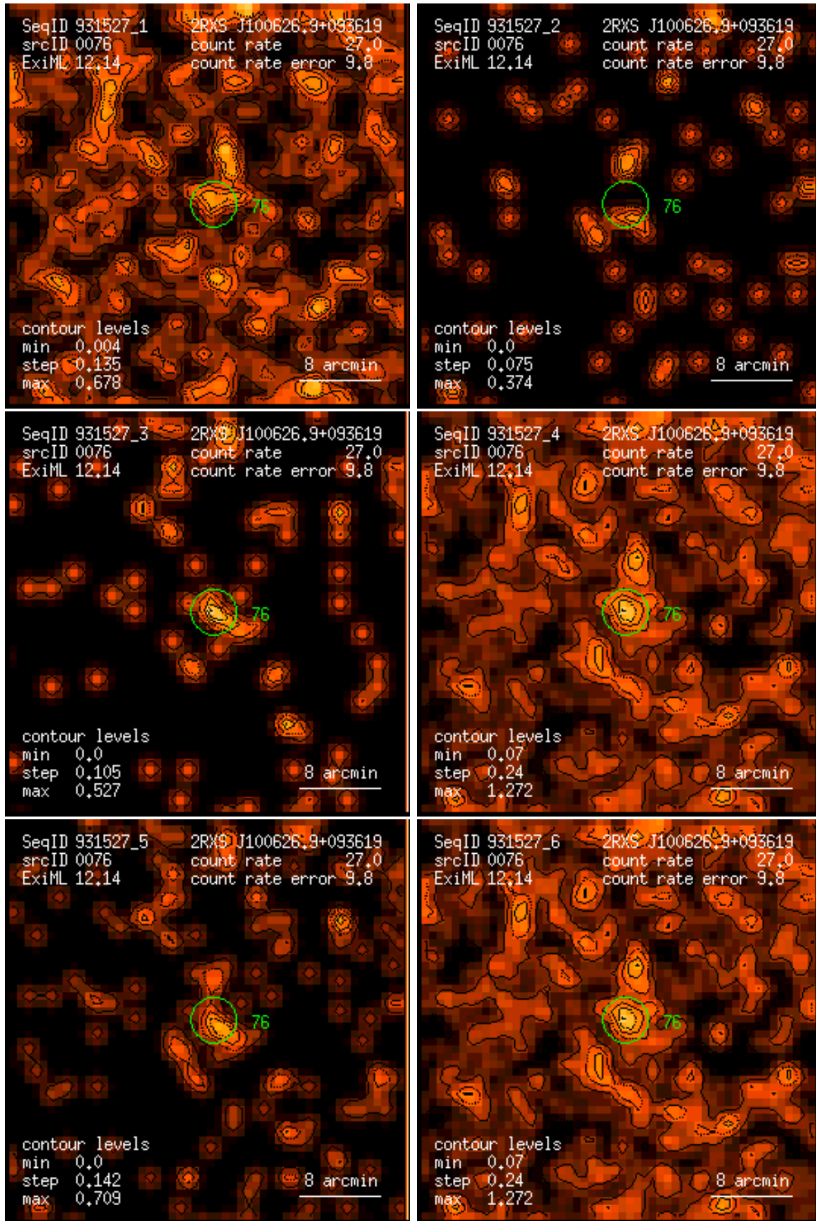
Figure 76: RASS 931527: detection 0076: band rate images, Gaussian filter: (1) PSPC channels 11 – 41, (2) 52 – 90, (3) 91 – 201, (4) 11 – 235, (5) 52 – 201, (6) 11 – 201. Broad band rates in counts/ks. Band rate contour levels in counts/ks/arcmin 2 .
