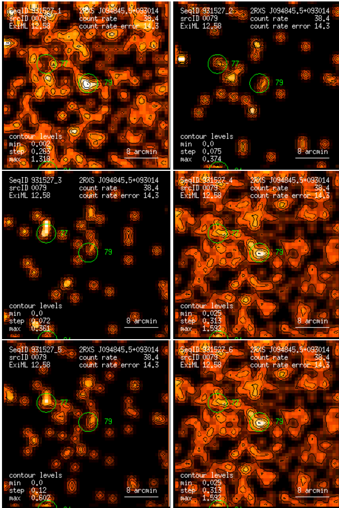
Figure 79: RASS 931527: detection 0079: band rate images, Gaussian filter: (1) PSPC channels 11 – 41, (2) 52 – 90, (3) 91 – 201, (4) 11 – 235, (5) 52 – 201, (6) 11 – 201. Broad band rates in counts/ks. Band rate contour levels in counts/ks/arcmin 2 .
