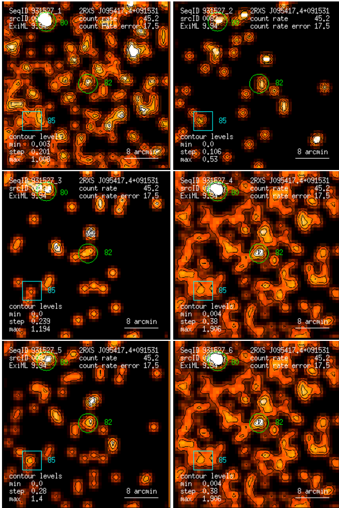
Figure 82: RASS 931527: detection 0082: band rate images, Gaussian filter: (1) PSPC channels 11 – 41, (2) 52 – 90, (3) 91 – 201, (4) 11 – 235, (5) 52 – 201, (6) 11 – 201. Broad band rates in counts/ks. Band rate contour levels in counts/ks/arcmin 2 .
