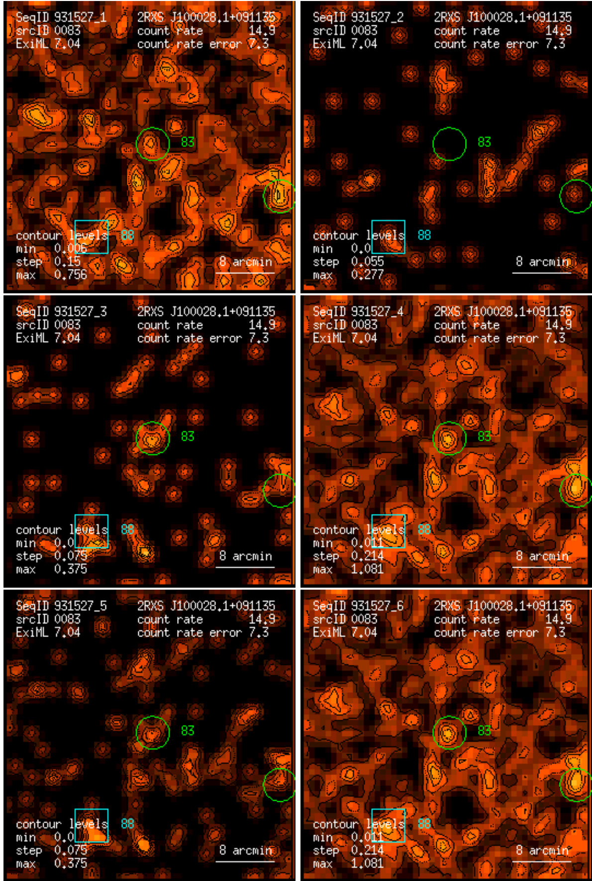
Figure 83: RASS 931527: detection 0083: band rate images, Gaussian filter: (1) PSPC channels 11 – 41, (2) 52 – 90, (3) 91 – 201, (4) 11 – 235, (5) 52 – 201, (6) 11 – 201. Broad band rates in counts/ks. Band rate contour levels in counts/ks/arcmin 2 .
