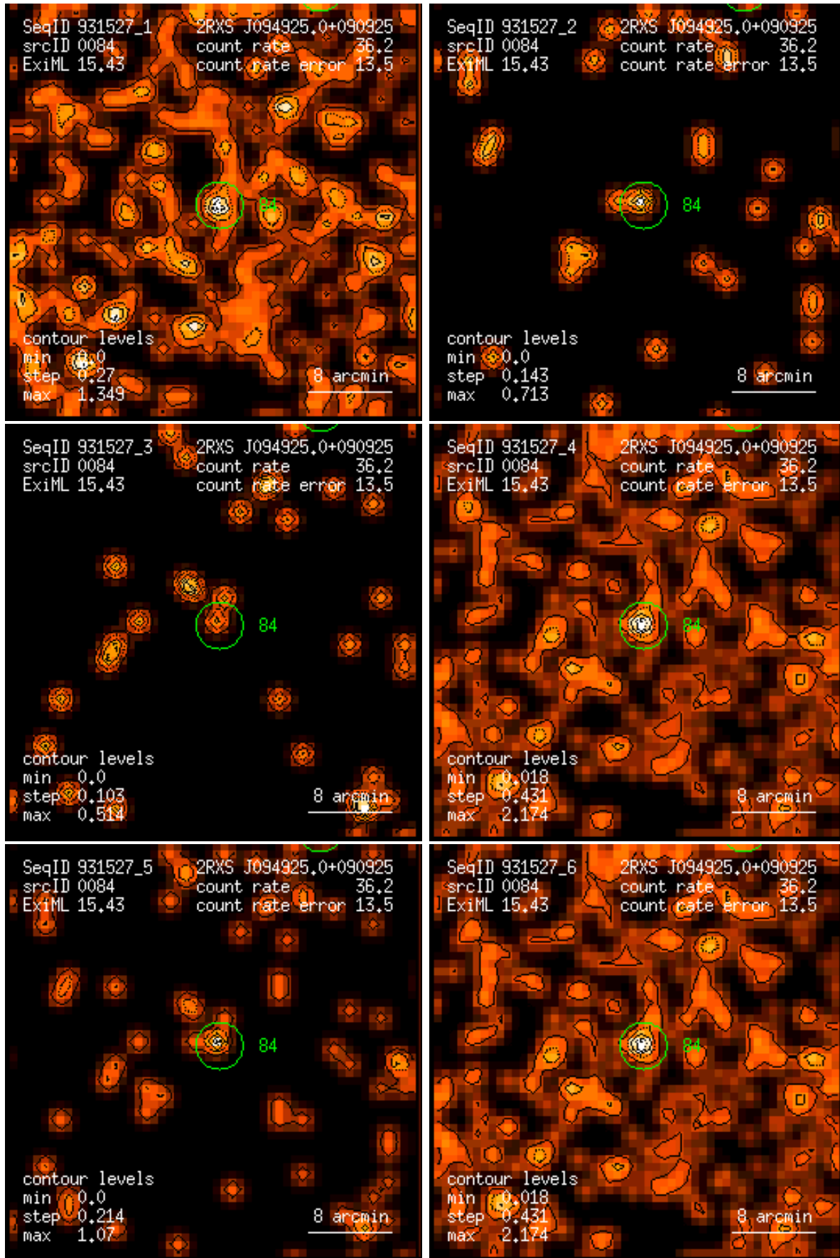
Figure 84: RASS 931527: detection 0084: band rate images, Gaussian filter: (1) PSPC channels 11 – 41, (2) 52 – 90, (3) 91 – 201, (4) 11 – 235, (5) 52 – 201, (6) 11 – 201. Broad band rates in counts/ks. Band rate contour levels in counts/ks/arcmin 2 .
