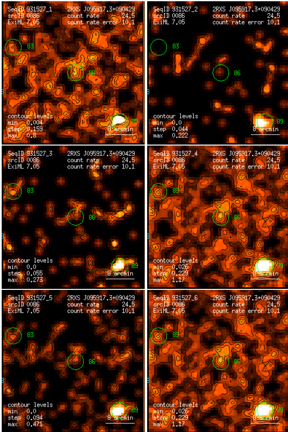
Figure 86: RASS 931527: detection 0086: band rate images, Gaussian filter: (1) PSPC channels 11 – 41, (2) 52 – 90, (3) 91 – 201, (4) 11 – 235, (5) 52 – 201, (6) 11 – 201. Broad band rates in counts/ks. Band rate contour levels in counts/ks/arcmin 2 .
