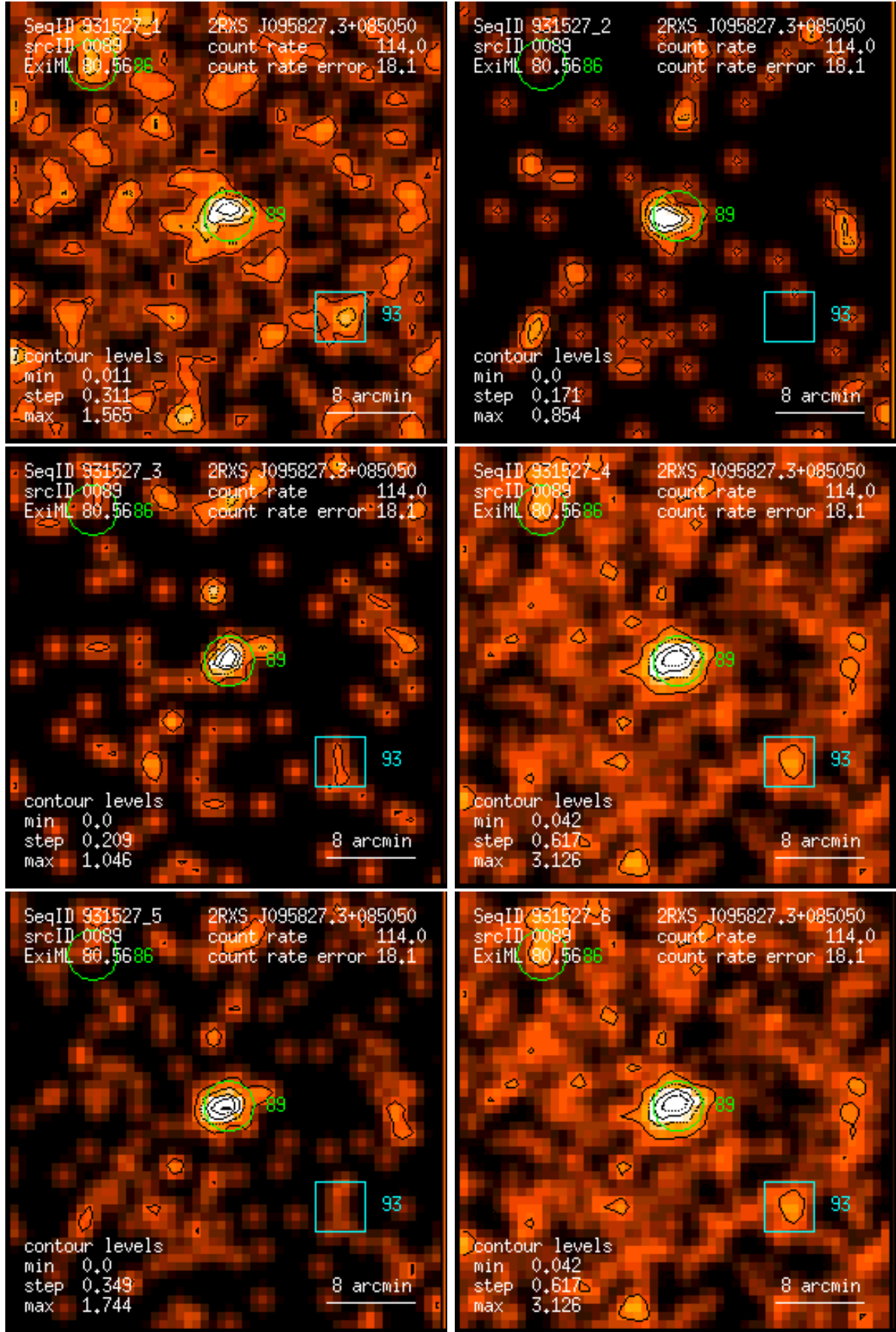
Figure 89: RASS 931527: detection 0089: band rate images, Gaussian filter: (1) PSPC channels 11 – 41, (2) 52 – 90, (3) 91 – 201, (4) 11 – 235, (5) 52 – 201, (6) 11 – 201. Broad band rates in counts/ks. Band rate contour levels in counts/ks/arcmin 2 .
