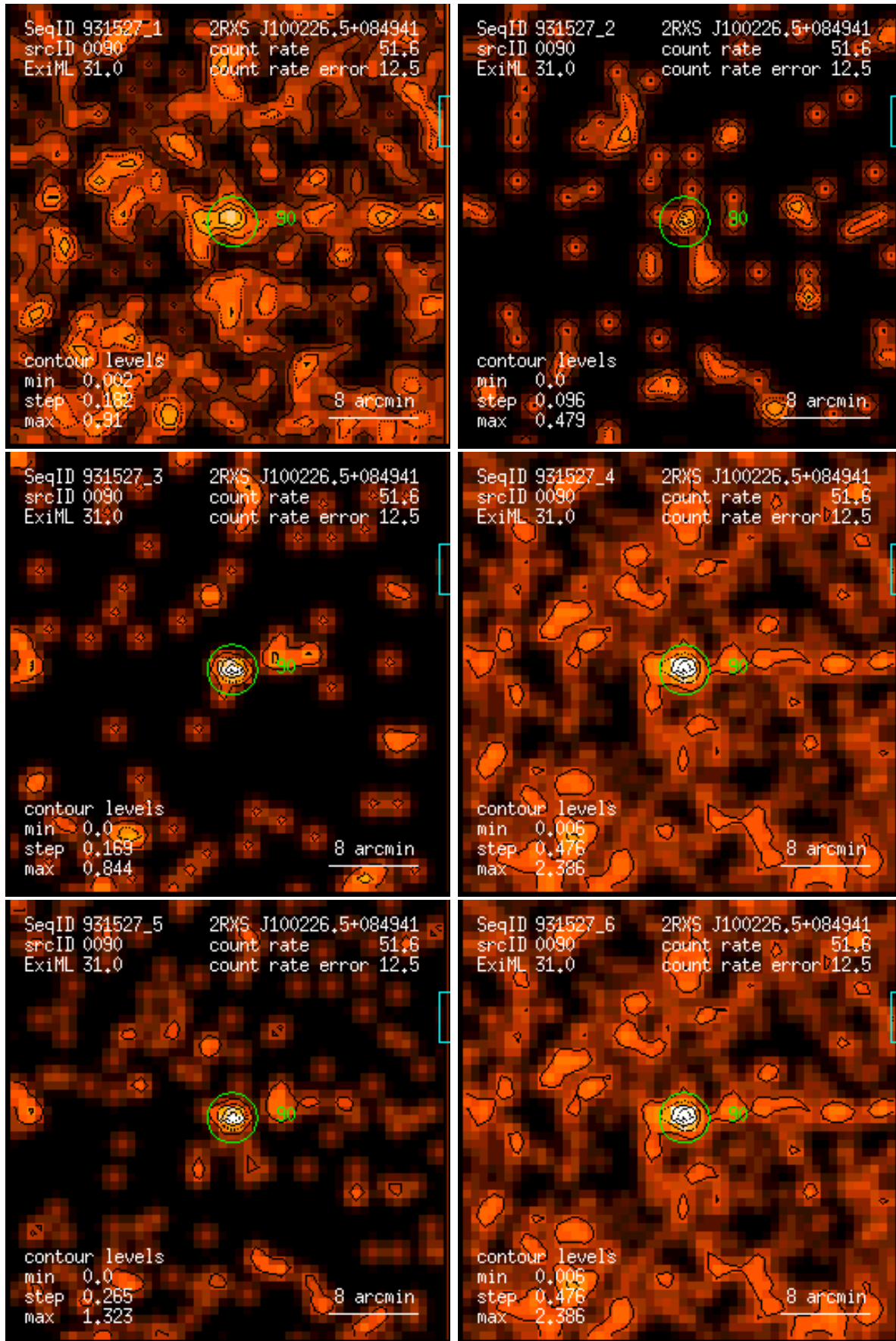
Figure 90: RASS 931527: detection 0090: band rate images, Gaussian filter: (1) PSPC channels 11 – 41, (2) 52 – 90, (3) 91 – 201, (4) 11 – 235, (5) 52 – 201, (6) 11 – 201. Broad band rates in counts/ks. Band rate contour levels in counts/ks/arcmin 2 .
