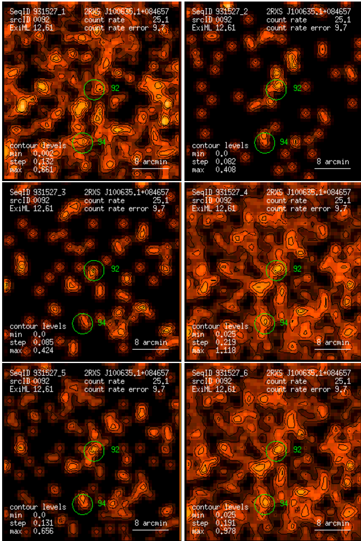
Figure 92: RASS 931527: detection 0092: band rate images, Gaussian filter: (1) PSPC channels 11 – 41, (2) 52 – 90, (3) 91 – 201, (4) 11 – 235, (5) 52 – 201, (6) 11 – 201. Broad band rates in counts/ks. Band rate contour levels in counts/ks/arcmin 2 .
