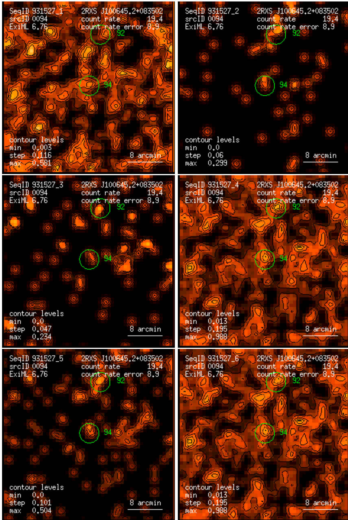
Figure 94: RASS 931527: detection 0094: band rate images, Gaussian filter: (1) PSPC channels 11 – 41, (2) 52 – 90, (3) 91 – 201, (4) 11 – 235, (5) 52 – 201, (6) 11 – 201. Broad band rates in counts/ks. Band rate contour levels in counts/ks/arcmin 2 .
