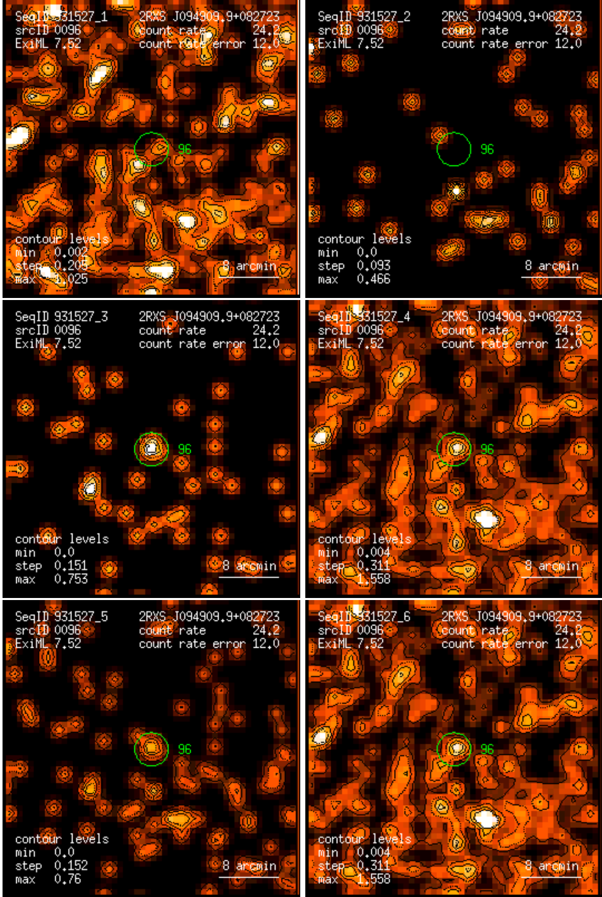
Figure 96: RASS 931527: detection 0096: band rate images, Gaussian filter: (1) PSPC channels 11 – 41, (2) 52 – 90, (3) 91 – 201, (4) 11 – 235, (5) 52 – 201, (6) 11 – 201. Broad band rates in counts/ks. Band rate contour levels in counts/ks/arcmin 2 .
