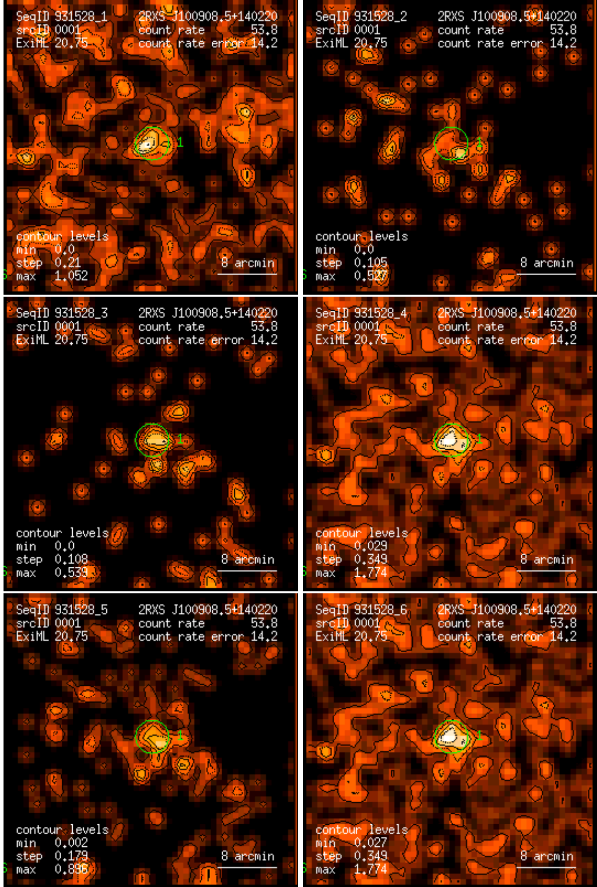
Figure 1: RASS 931528: detection 0001: band rate images, Gaussian filter: (1) PSPC channels 11 – 41, (2) 52 – 90, (3) 91 – 201, (4) 11 – 235, (5) 52 – 201, (6) 11 – 201. Broad band rates in counts/ks. Band rate contour levels in counts/ks/arcmin 2 .
