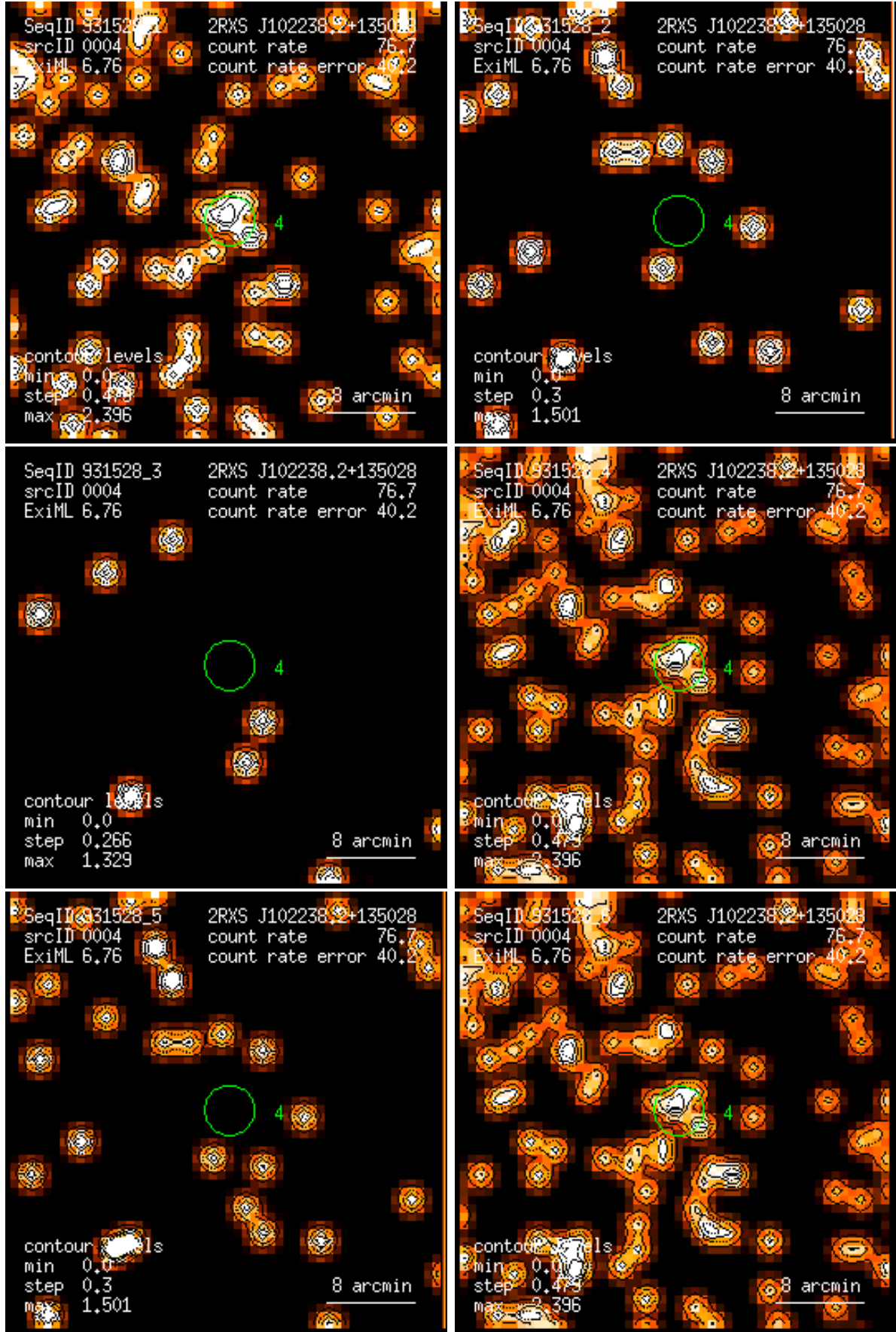
Figure 4: RASS 931528: detection 0004: band rate images, Gaussian filter: (1) PSPC channels 11 – 41, (2) 52 – 90, (3) 91 – 201, (4) 11 – 235, (5) 52 – 201, (6) 11 – 201. Broad band rates in counts/ks. Band rate contour levels in counts/ks/arcmin 2 .
