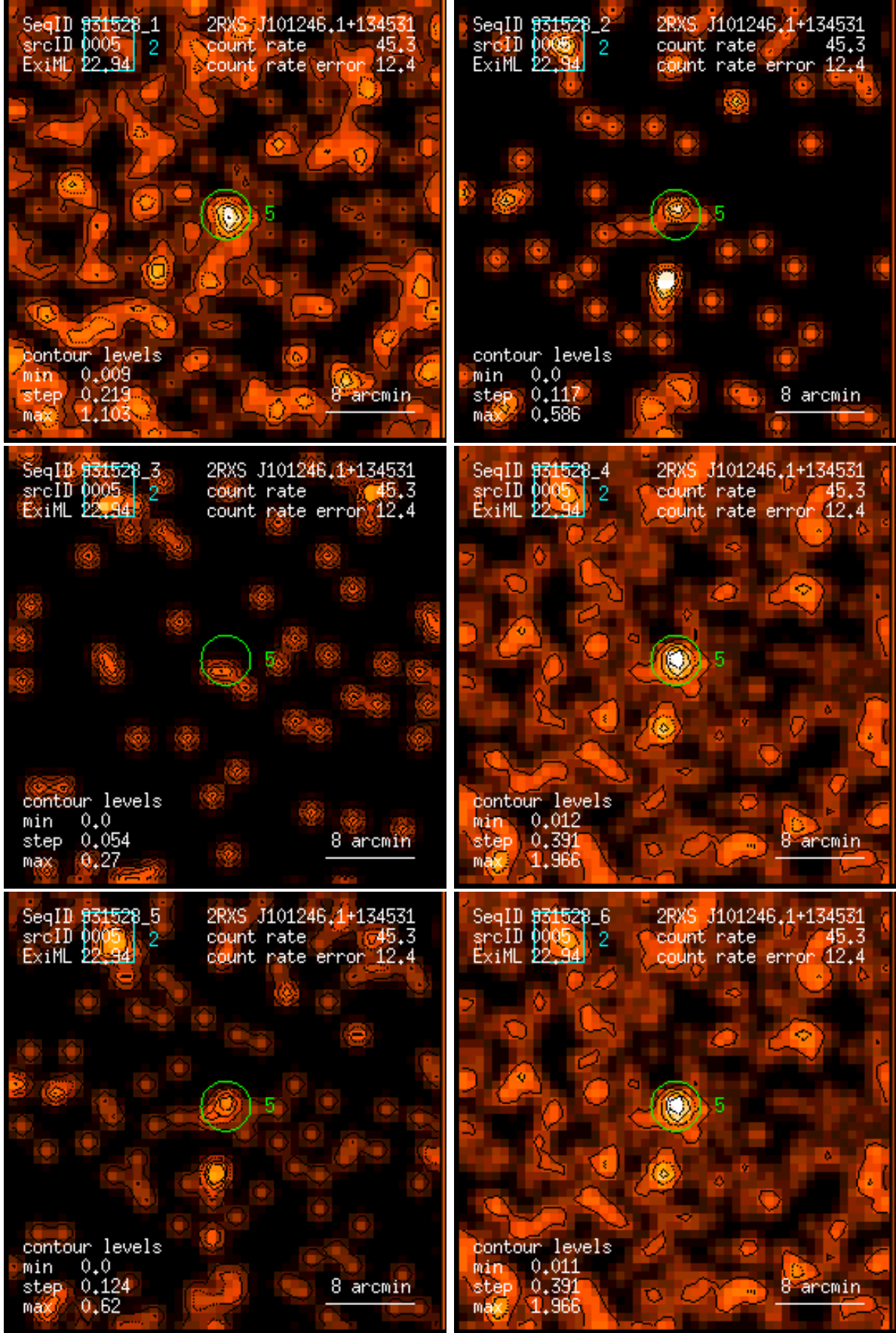
Figure 5: RASS 931528: detection 0005: band rate images, Gaussian filter: (1) PSPC channels 11 – 41, (2) 52 – 90, (3) 91 – 201, (4) 11 – 235, (5) 52 – 201, (6) 11 – 201. Broad band rates in counts/ks. Band rate contour levels in counts/ks/arcmin 2 .
