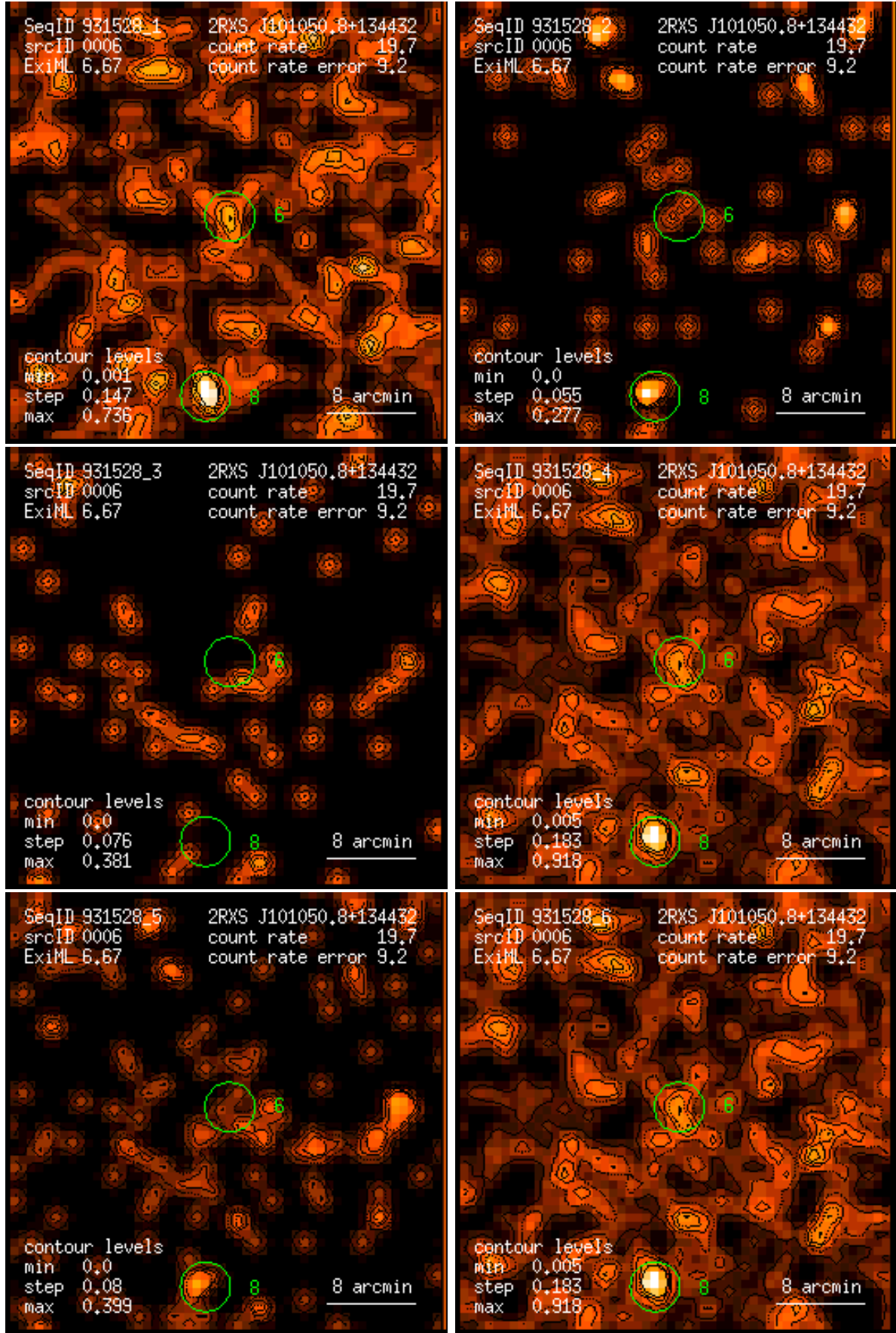
Figure 6: RASS 931528: detection 0006: band rate images, Gaussian filter: (1) PSPC channels 11 – 41, (2) 52 – 90, (3) 91 – 201, (4) 11 – 235, (5) 52 – 201, (6) 11 – 201. Broad band rates in counts/ks. Band rate contour levels in counts/ks/arcmin 2 .
