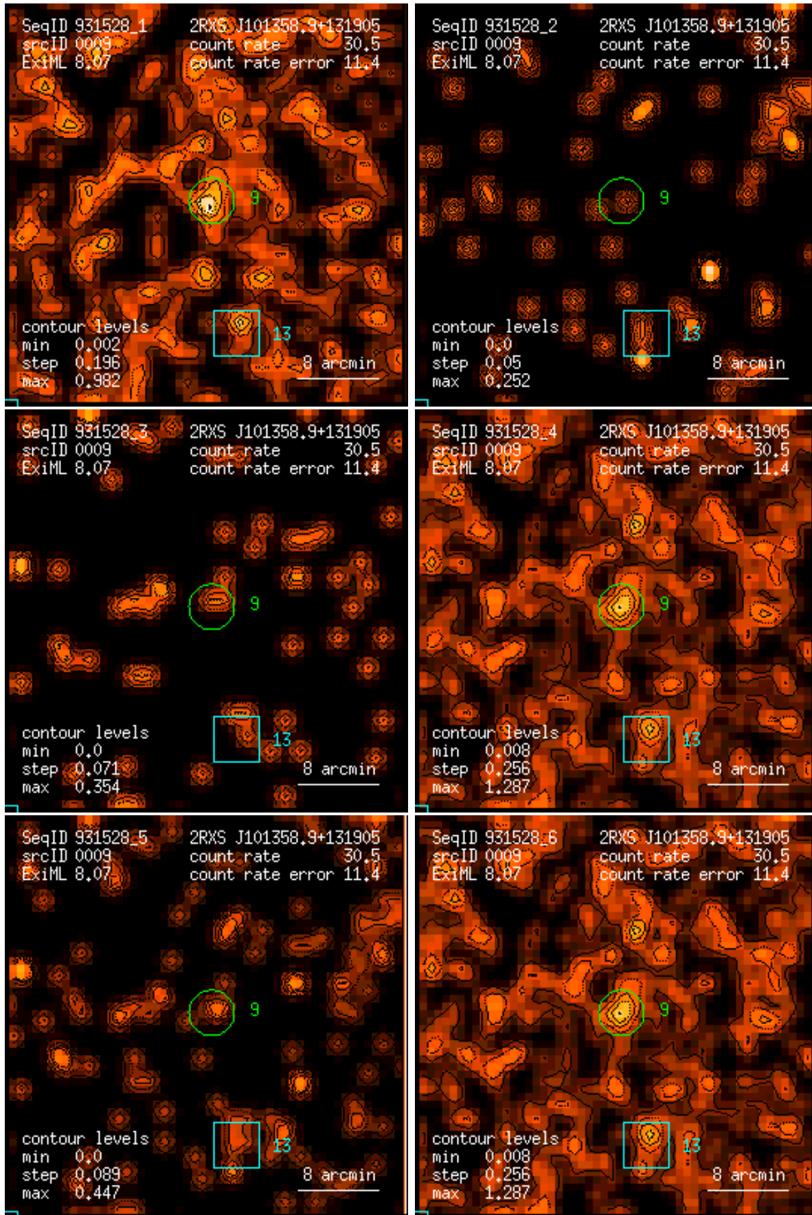
Figure 9: RASS 931528: detection 0009: band rate images, Gaussian filter: (1) PSPC channels 11 – 41, (2) 52 – 90, (3) 91 – 201, (4) 11 – 235, (5) 52 – 201, (6) 11 – 201. Broad band rates in counts/ks. Band rate contour levels in counts/ks/arcmin 2 .
